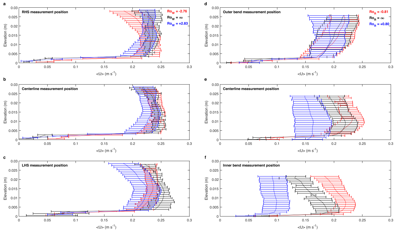
Figure 5. Time-averaged downstream velocity profiles of the bottom 0.028 m (from ADVP1) at three measurement locations across the channel for (a), (b), (c) the straight section ( Ro_W = -2.76, \infty, +2.83 corresponding to experiments 3X1S, 6X1EQ, and 3X1N) and (d), (e), (f) the bend apex section ( Ro_R = -0.81, \infty, +0.8 corresponding to experiments 3X2S, 6X2EQ, and 3X2N). Error bars represent one standard error from the mean (68.2% confidence intervals) and were estimated using the equations provided by Benedict and Gould (1996).
