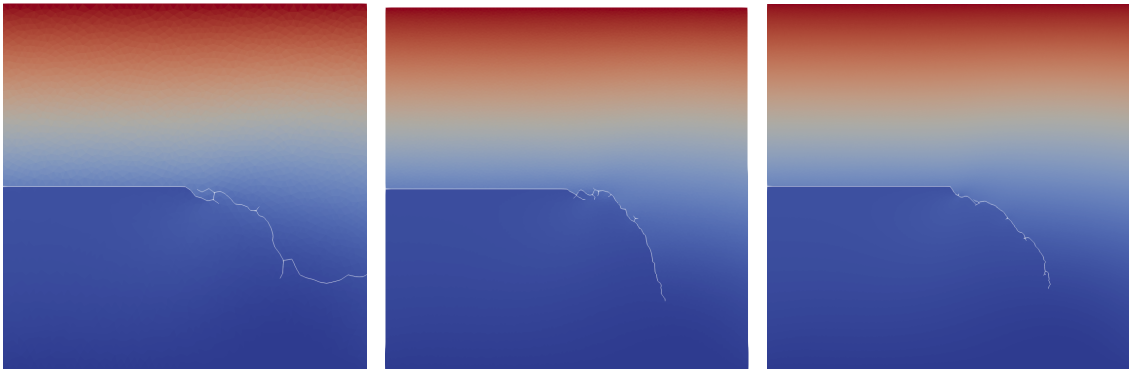
Figure 15: Single-edge notched shear test: u_x in colors and crack path in white, u_D = 0.2\text{mm} . Left: coarse mesh. Middle: fine mesh. Right: finest mesh.
