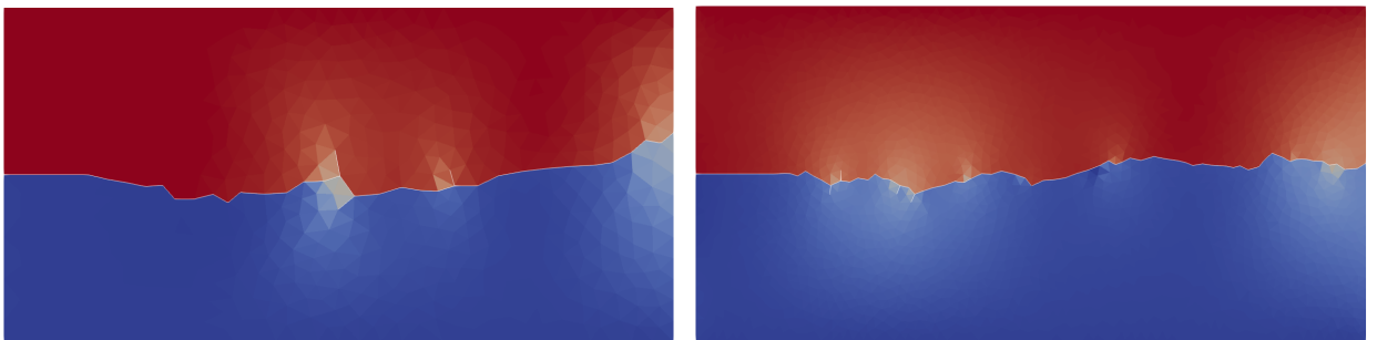
Figure 13: Opening mode: u_y in colors and crack path in white on a unstructured mesh. Left: coarse mesh, u_D = 2.5\text{mm} . Right: fine mesh, u_D = 3.4\text{mm} .
