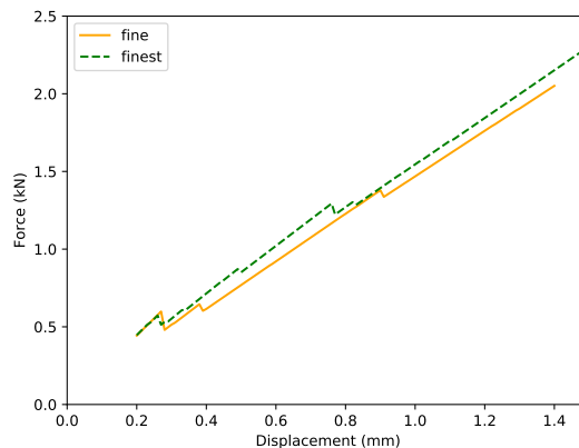
Figure 20: Notched plate with a hole: load-displacement curves.
