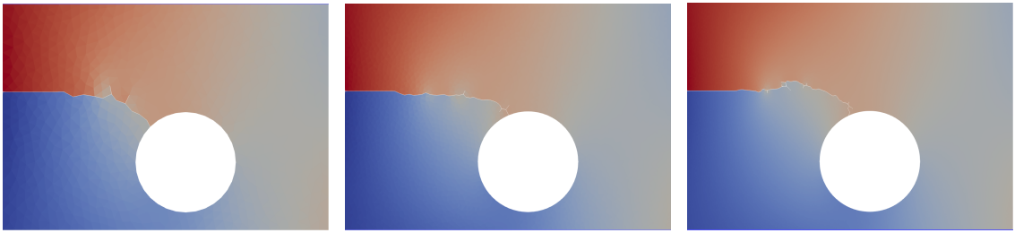
Figure 18: Notched plate with a hole: u_y in colors and crack path in white (zoom around the main hole). Left: coarse mesh, u_D = 0.65\text{mm} . Middle: fine mesh, u_D = 1.4\text{mm} . Right: finest mesh, u_D = 3.0\text{mm} .
