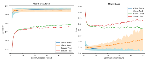
Figure 5. CNN performance vs com. rounds (REALWORLD).
