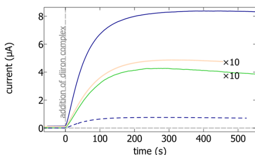
Fig. 1: Electrochemically-monitored time-resolved artificial maturation of anaerobically prepared films of Me apo-hydrogenase, under three distinct conditions: MET in a thin polymer film (green, enlarged ten times) or in a thicker polymer film (dark blue), and DET (orange, enlarged ten times). The maturation was also monitored with another thick polymer film of apo-hydrogenase exposed to air for two hours (dark blue, dashed line, see the optimization procedure in SI). In all experiments, the maturation is detected as an increase in hydrogen oxidation current after 53 nM [\text{Fe}_2(\text{adt})(\text{CO})_4(\text{CN})_2]^{2-} is added to the electrochemical cell under anaerobic conditions, at t=0 s. E=-160\text{mV} vs SHE, 40^\circ\text{C} , pH 7, 1 atm. \text{H}_2 , \omega = 3000 rpm.
