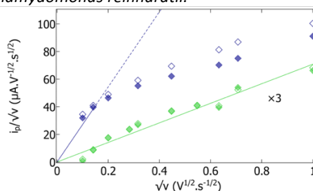
Fig. 2. Evaluation of the thin (green, enlarged three times) and thick (dark blue) hydrogenase/polymer films by cyclic voltammetry under non-catalytic conditions (under argon). Plot of anodic (open) and cathodic (full) peak currents divided by the square root of scan rate ( \sqrt{v} ), against \sqrt{v} . A straight line through the origin is expected when the film is so thin that all viologen moieties are oxidized or reduced in each sweep.
