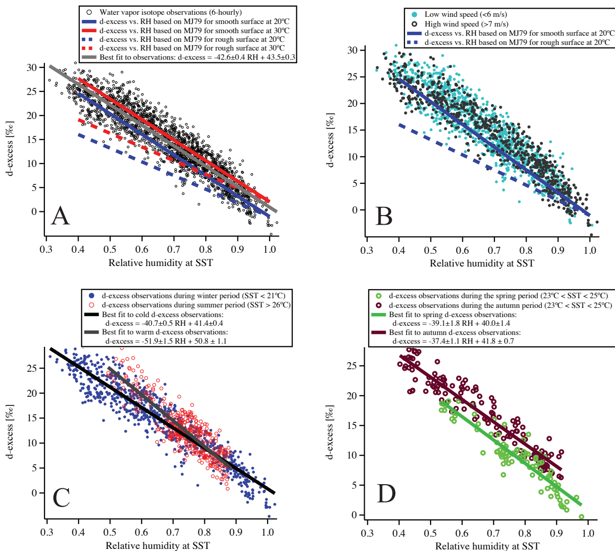
Figure 11. (A) Complete set of 6-hourly observations of d-excess vs. relative humidity ( \text{RH}_{\text{SST}} ) at sea surface temperature (black dots), with a best fit (grey line). Results from the theory of MJ79 are displayed for a rough and smooth surface, and for SST of 20 and 30 °C. (B) The complete set of 6-hourly observations of d-excess vs. \text{RH}_{\text{SST}} separated into calm (< 6 m s -1 – cyan dots) and strong winds (> 7 m s -1 – grey dots). MJ79 calculations are shown for a rough and smooth surface at 20 °C. (C) Observations collected during winter (defined as SST < 21 °C – blue dots) and summer (defined as SST > 26 °C – red dots) period. The best linear fits to winter and summer observations are shown as black and grey solid lines. (D) Observations collected during the spring (23 °C < SST < 25 °C – green dots) and autumn (23 °C < SST < 25 °C – brown dots) period. Best linear fits to the spring and autumn period are shown as, respectively, green and brown solid lines.
