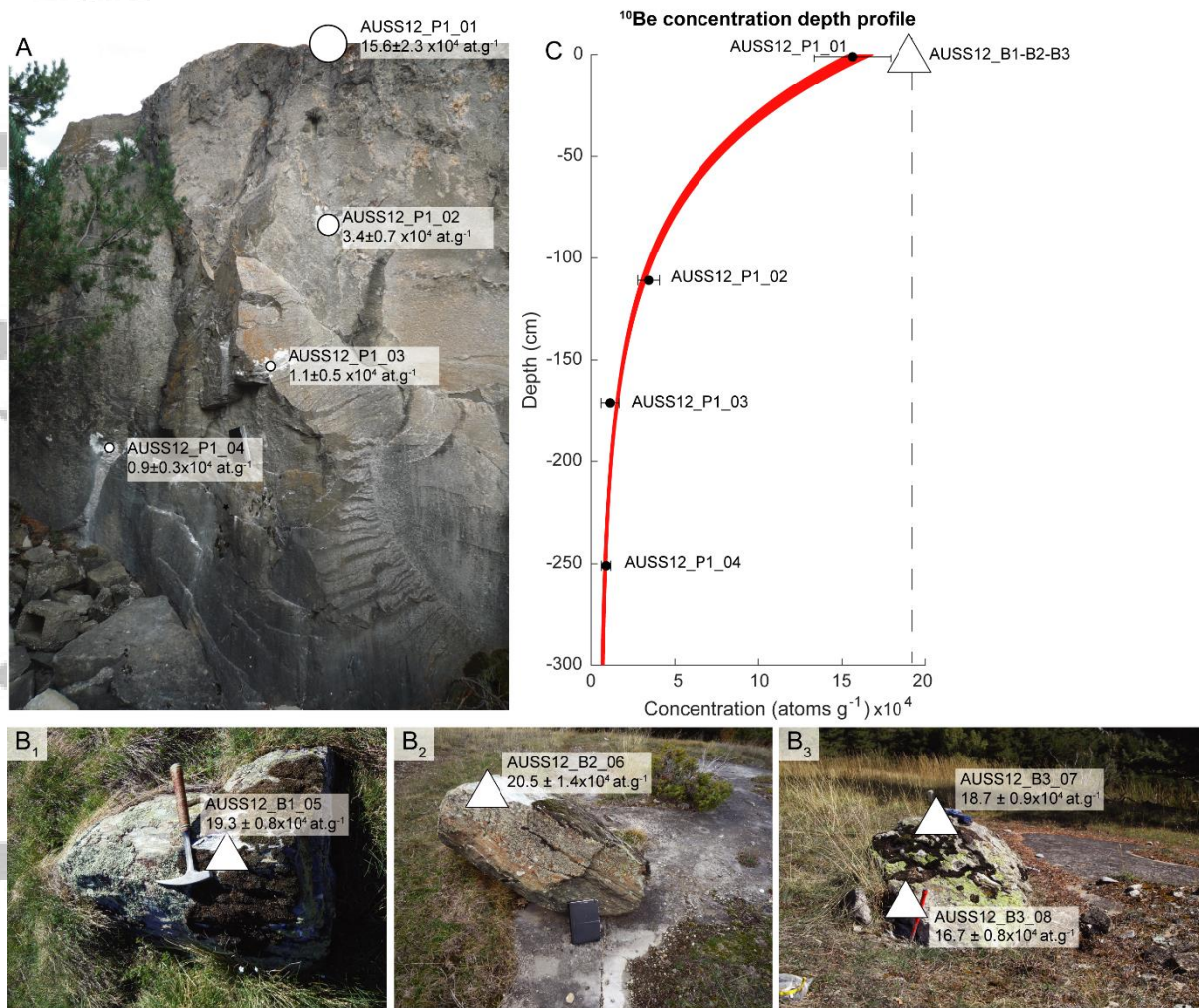
Figure 7: Aussois site: Sample locations and ^{10}\text{Be} concentration in erratic boulders (AUSS12_B1, AUSS12_B2 and AUSS12_B3) and in polished surface (AUSS12_P1). A) Vertical cross-section for the sampling polished bedrock associated with depth locations of the samples. B) Sample locations of the three different erratic boulders (B 1 , B 2 , B 3 ). The circles and triangles illustrate the sampling positions and their sizes are dependent on the ^{10}\text{Be} concentrations of the samples. C) Results from the Monte-Carlo concentration-depth profile simulation of the polished bedrock; 2\sigma profile solution spaces (red line), measured ^{10}\text{Be} concentration samples with associated uncertainties (filled black circles and error bars). For comparison, we report the average surface ^{10}\text{Be} concentration (dashed line) in the three erratic boulders (white triangle). The input and output parameters of the concentration-depth profile simulation are reported in Table 2.
