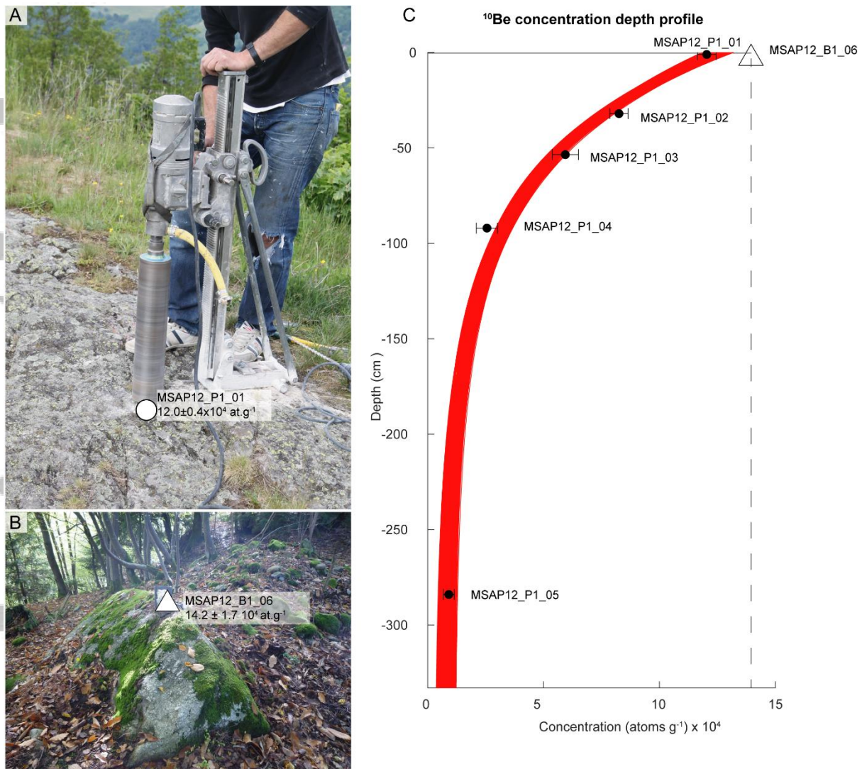
Figure 6: Montsapey site: Sample locations and ^{10}\text{Be} concentrations in erratic boulder (MSAP12_B1_06) and polished surface (MSAP12_P1). A) Sampling of the polished bedrock using a drilling machine (model DK52, brand WEKA), equipped with a mining drill with a diameter of 90 mm. B) erratic boulder and the sample position. The circles and triangles illustrate the sampling positions and their sizes are dependent on the ^{10}\text{Be} concentrations of the samples. C) Results from the Monte-Carlo concentration-depth profile simulation of the polished bedrock; 2\sigma profile solution spaces (red line), measured ^{10}\text{Be} concentration samples with associated uncertainties (filled black circles and error bars). For comparison, we report the surface ^{10}\text{Be} concentration (dashed line) in the erratic boulder (white triangle). The input and output parameters of the concentration-depth profile simulation are reported in Table 2.
