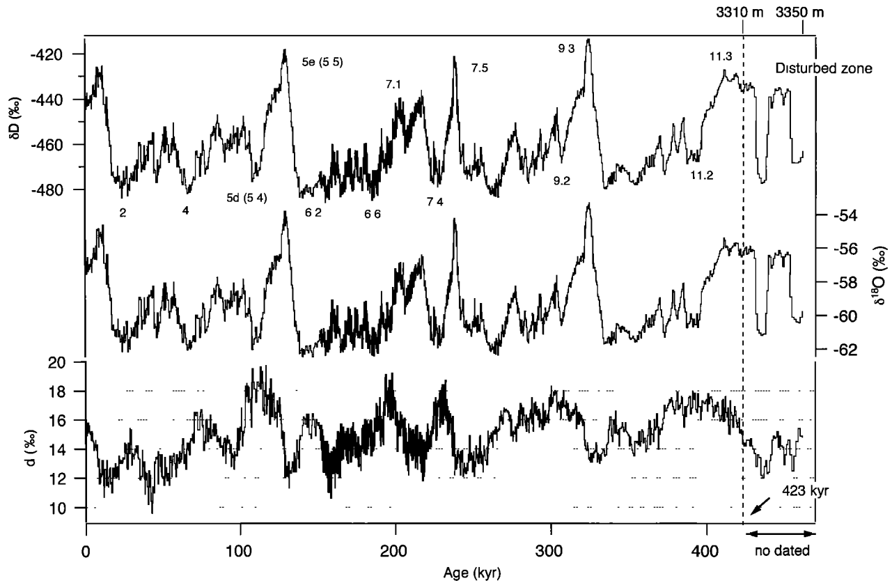
Figure 2. Times series of \delta D , \delta^{18}O and deuterium excess. These records combine data available down to 2083m [Vimeux et al. , 1999] and new measurements performed along two deep cores : 4G from 2083m to 2755m and 5G down to 3350m with 1m depth resolution. Data are presented at 1m depth resolution excepting the last climatic cycle, which is presented at a 5m depth resolution. The temporal resolutions are always smaller than 500 years. Deuterium excess experimental accuracy is \pm 0.7\text{‰} ( \pm 0.5\text{‰} for \delta D and \pm 0.05\text{‰} for \delta^{18}O ) excepting from 1413m to 2083m at \pm 1.3\text{‰} . Down to 3310m we used the glaciological timescale GT4 [Petit et al. , 1999], the accuracy of which is estimated to be always better than \pm 15 kyr (kiloyears) all over the profile. GT4 provides an age of 423 kyr at the depth of 3310m [Petit et al. , 1999].
