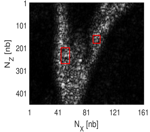
Fig. 1. Simulated B-mode image. Note that N_z [nb] and N_x [nb] denote the lateral and axial distances in number of samples.
