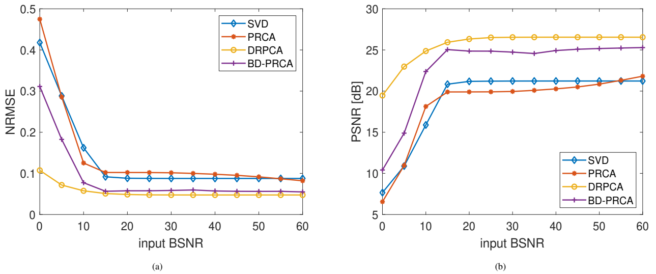
Fig. 5. Quantitative measures of different retrieval techniques as a function of input BSNR in the noisy case, in terms of: (a) NRMSE; (b) PSNR.
