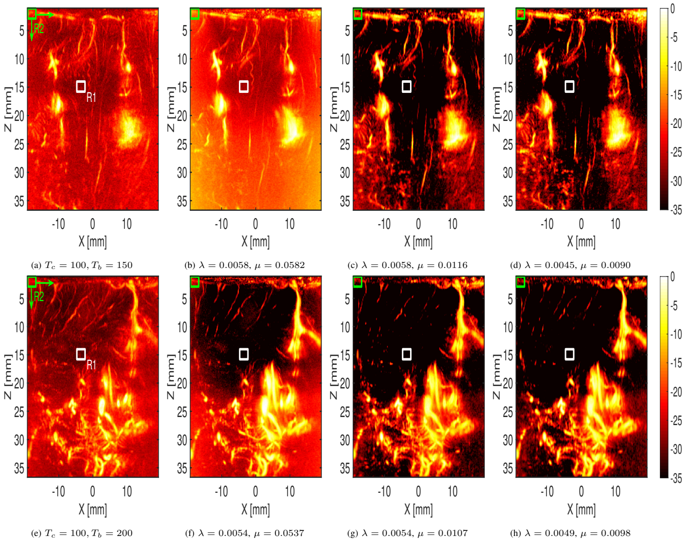
Fig. 6. First row panels: Power Doppler images computed on the healthy brain dataset by respectively using: (a) SVD; (b) PRCA; (c) DRPCA; (d) BDRPCA. Second row panels: the same as first row panel but for the tumor dataset. All the images are displayed with a dynamic range of 35 dB. The arrows mean that R_2 is successively moved patch by patch in both directions and combined with R_1 in order to compute CR values. The best possible hyperparameters associated with each blood recovery technique are also provided in each plot.
