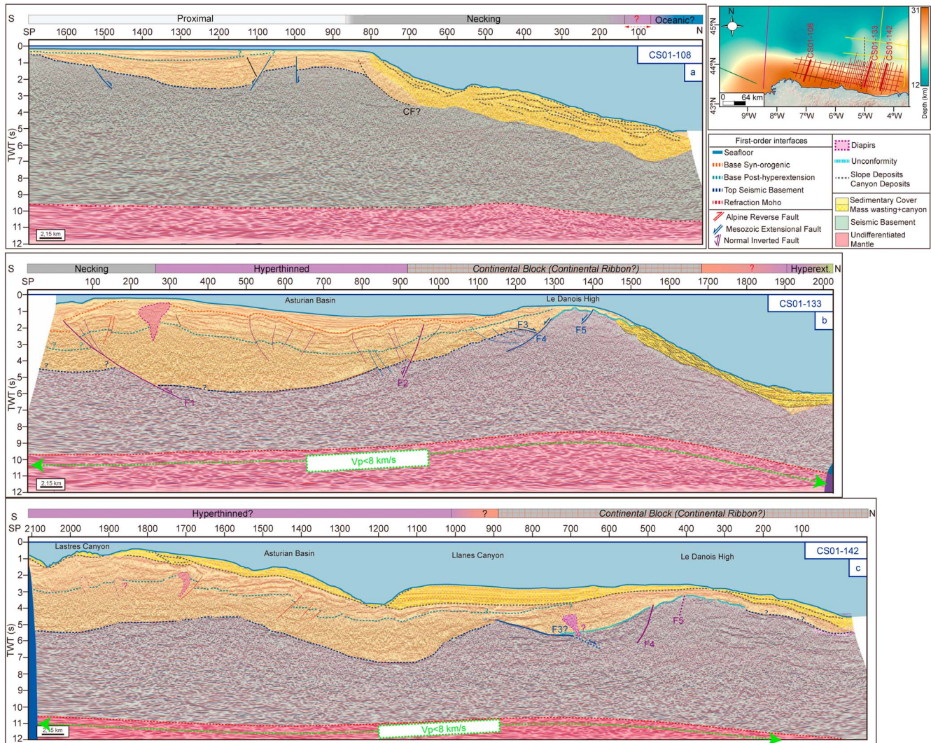
Figure 3. Representative time migrated seismic reflection lines crossing the North Iberian margin at three different longitudes, showing the seismic interpretation of the main structures, the first-order interfaces and, on top, the interpreted rift domains. (a) CS01-108 seismic line at the westernmost area, (b) CS01-133 section at the central part of the margin, and (c) CS01-142 seismic profile located in the easternmost part of the studied zone. The seismic Moho and the presence of anomalous mantle velocities ( V_p < 8 km/s) have been estimated using the velocity models of Ayarza et al. (1998), Fernández-Viejo et al. (1998, 2012), and Ruiz (2007). The inset map shows the location of the reflection lines within the seismic data set (red). The map also displays the Moho depth and the distribution of the wide-angle profiles used to estimate its position. IAM-12 profile, displayed in pink, ESCIN-3.1, shown in green, and ESCIN-4, delineated with a dashed black line, are from Fernández-Viejo et al. (1998); ESCIN-3.3, displayed in black, is from Ayarza et al. (1998); MARCONI profiles, shown in yellow (MARCONI-1 and MARCONI-6 from west to east, and MARCONI-4 and MARCONI-8 from north to south), are from Ruiz (2007). CF: Cantabrian fault from Fernández-Viejo et al. (2014). F1 to F5 faults in the Asturian Basin from Cadenas and Fernández-Viejo (2017). The uninterpreted version of the three seismic profiles is provided as supplementary information (Figure S1).
