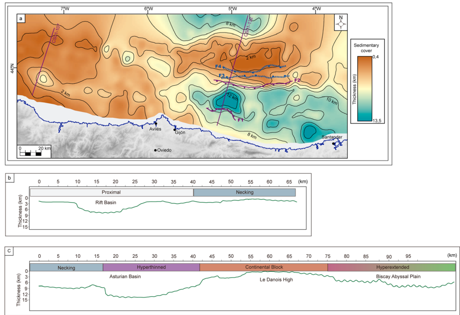
Figure 9. Sediment thickness within the central and western North Iberian margin. (a) Map of isolines showing thickness variations of the sedimentary cover, based on the depth-converted first-order interfaces interpreted in this study. The map shows the location of the sections displayed in Figures 9b and 9c. (b) Section illustrating sediment thickness variations in the western North Iberian margin along the CS01-107 seismic profile. (c) Section showing sediment thickness variations in the central North Iberian margin along the CS01-132 seismic line. Interpreted rift domains are displayed on top of the sections.
