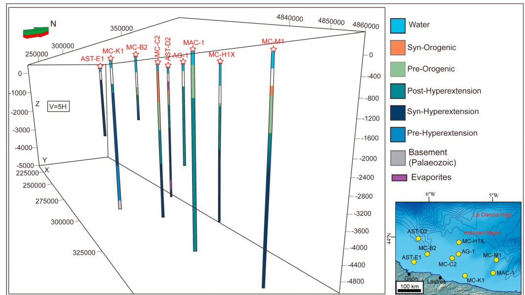
Figure 7. 3-D view of nine representative boreholes drilled in the Asturian Basin showing thickness variations of the main tectono-stratigraphic units along the whole area. The stratigraphic information has been taken from the well reports. See Lanaja (1987), Gutiérrez-Claverol and Gallastegui (2002), and Cadenas and Fernández-Viejo (2017) for stratigraphic columns. We defined the main seismo-stratigraphic units displayed along the boreholes based on seismic to well ties. This figure is provided on a larger scale as supporting information (Figure S3).
