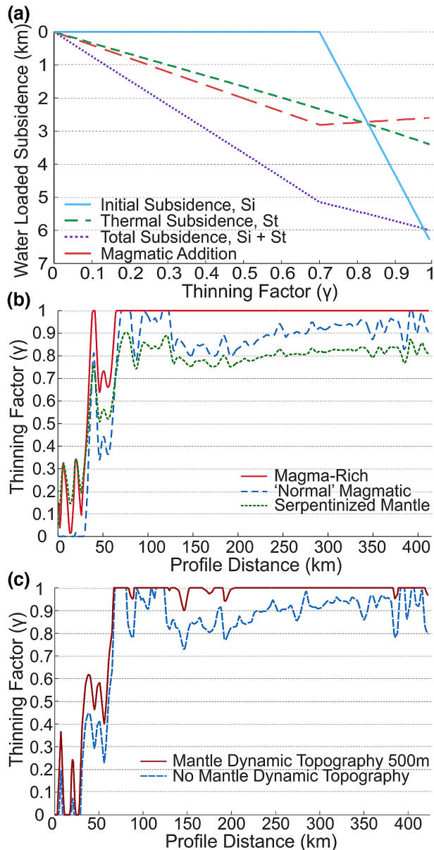
Figure 5. Subsidence analysis: (a) Water-loaded subsidence as a function of thinning factor predicted from McKenzie (1978) modified to include 'normal' decompression melting. (b) Lithosphere thinning factors calculated from subsidence analysis for INE1-1000 for a magma-rich, a 'normal' magmatic solution and a serpentinized mantle solution. (c) 'Normal' magmatic thinning factor from subsidence analysis showing the effect of 500 m of mantle dynamic topography.
