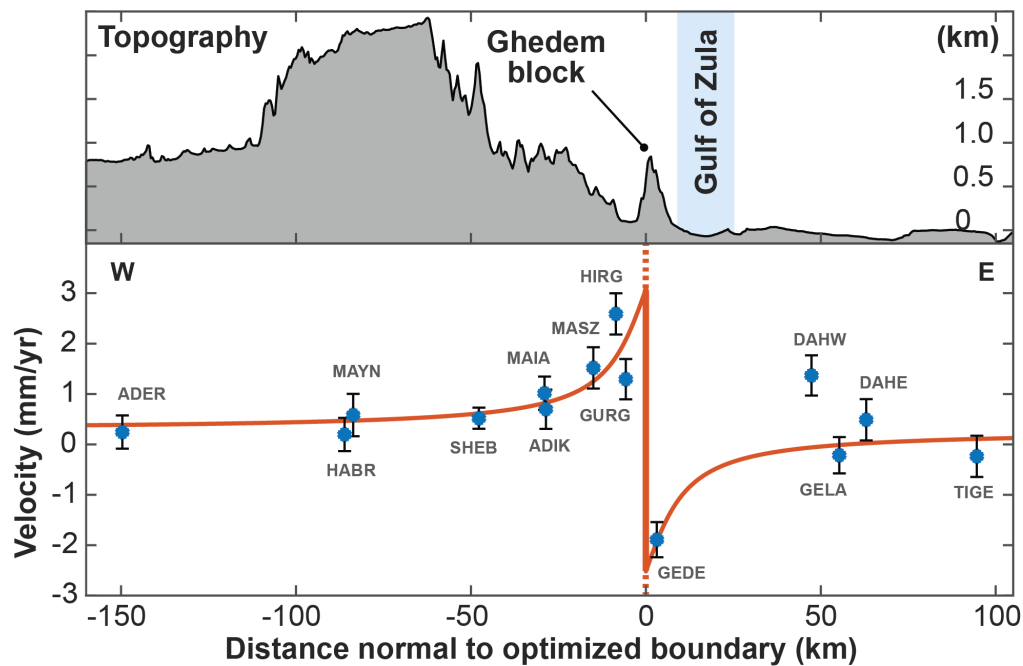
Figure 7. GPS velocities (blue circles with 1- \sigma bars) in the \sim N84°E direction (see Fig. 6) after the Danakil-Nubia relative block motion has been removed, in comparison to the best-fitting inter-rifting model prediction (solid red line) and the profile topography (top).
