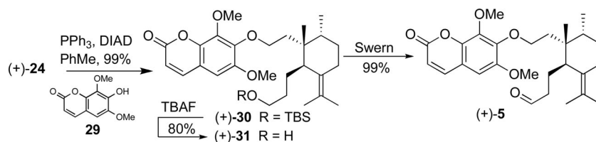
Scheme 9. Completion of the synthesis of the secodriol analogue (+)-26.
