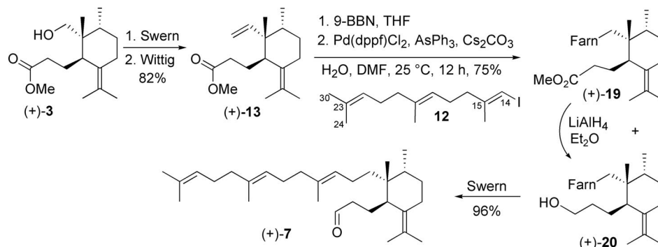
Scheme 5. Improved synthesis of marneral [ (+)-3 ] (Farn represents the C13–C30 farnesyl chain, squalene numbering).
