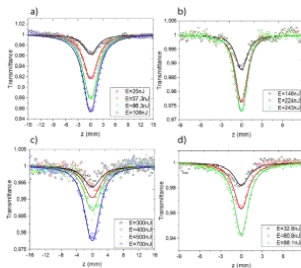
Figure 5. Nonlinear transmittance of 5 (a,b) and 6 (c,d) at 1300 (a,c) and 1550 nm (b, d). The open circles indicate the experimental points at a given incident pulse energy. The line represents the fit using eq.1 enabling to extract the 2PA and ESA cross-sections.
