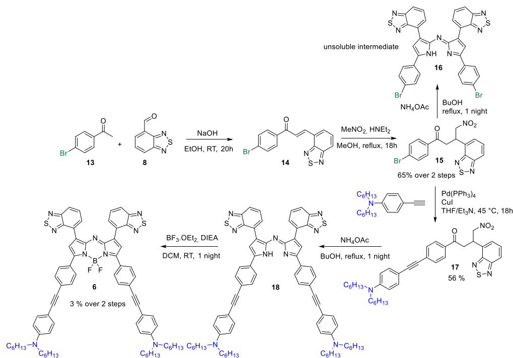
Scheme 2. Synthetic procedure for the preparation of 6 .
