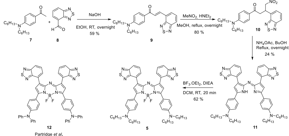
Scheme 1. Synthetic procedure for the preparation of 5 . In the left corner is represented the previously published dye ( 12 ). [19]
