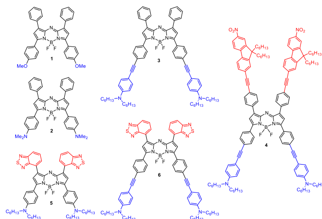
Figure 1. Structures of the different aza-BODIPY dyes designed for advanced photonic applications.
