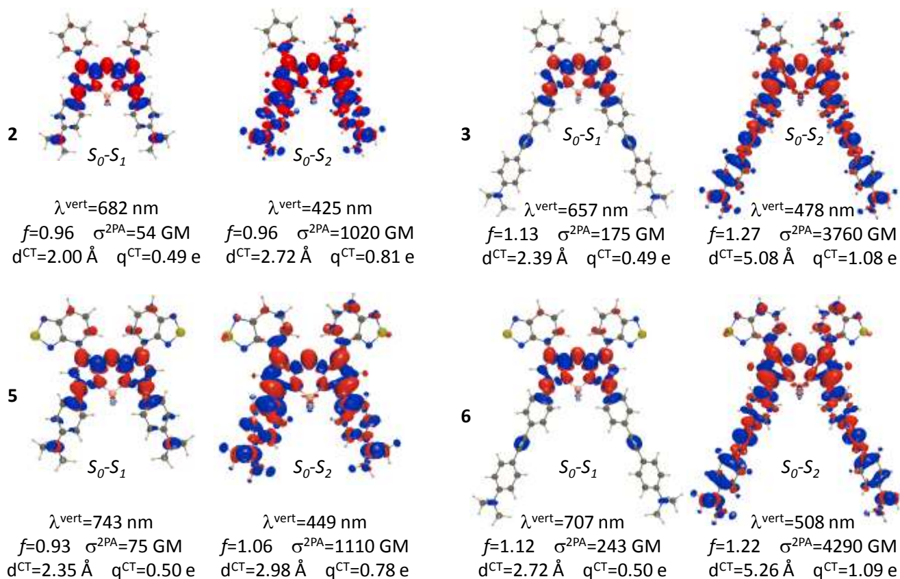
Figure 4. Summary of the main theoretical results. We represent for the key transitions, the density difference plots (red: increase of density, blue: decrease of density upon excitation, 0.0008 isovalue), and provide the vertical 1PA transition energies and oscillator strengths, as well as the 2PA cross sections. We also give the CT distance and charge computed using Le Bahers' model. [24]
