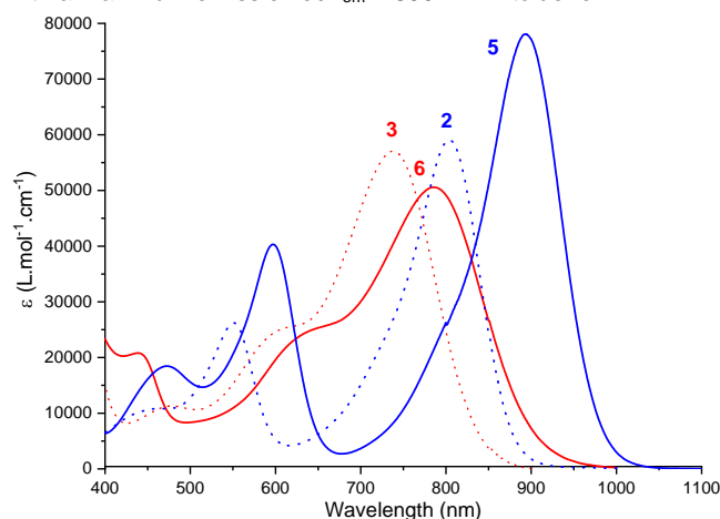
Figure 2. Molar absorptivity comparison of aza-BODIPYs 5 and 6 featuring BTZ substituents (straight line) with related dyes 2 and 3 featuring phenyl substituents (dotted lines) at the 1,7 positions. Spectra were recorded at room temperature in diluted DCM solution.
