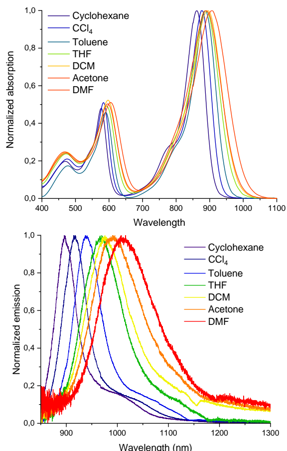
Figure 3. Normalized absorption (top) and emission (bottom) of 5 in different solvents indicated in inset.
