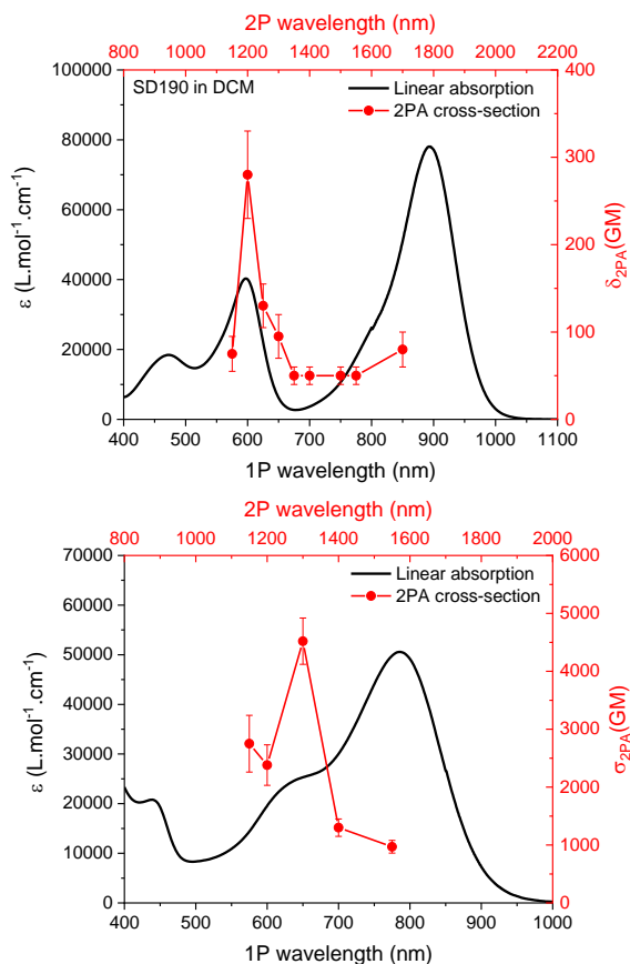
Figure 6. Comparison between linear absorption (black line and corresponding black scale) and two-photon absorption (red dot and corresponding red scale) for compounds 5 (top) and 6 (bottom).
