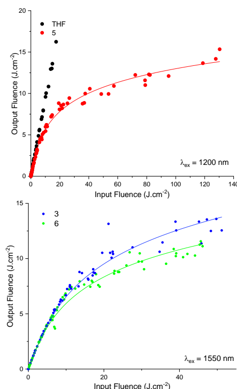
Figure 7. Top: OPL experiment for compound 5 in THF, (red circles) and pure THF (black circles) at 1200 nm. Bottom: OPL experiments for compounds 3 (blue) and 6 (green) at 1550 nm in \text{CCl}_4 . All measurements were done in 50 mM solutions, performed in a f/5 set-up and 4 ns pulses.
