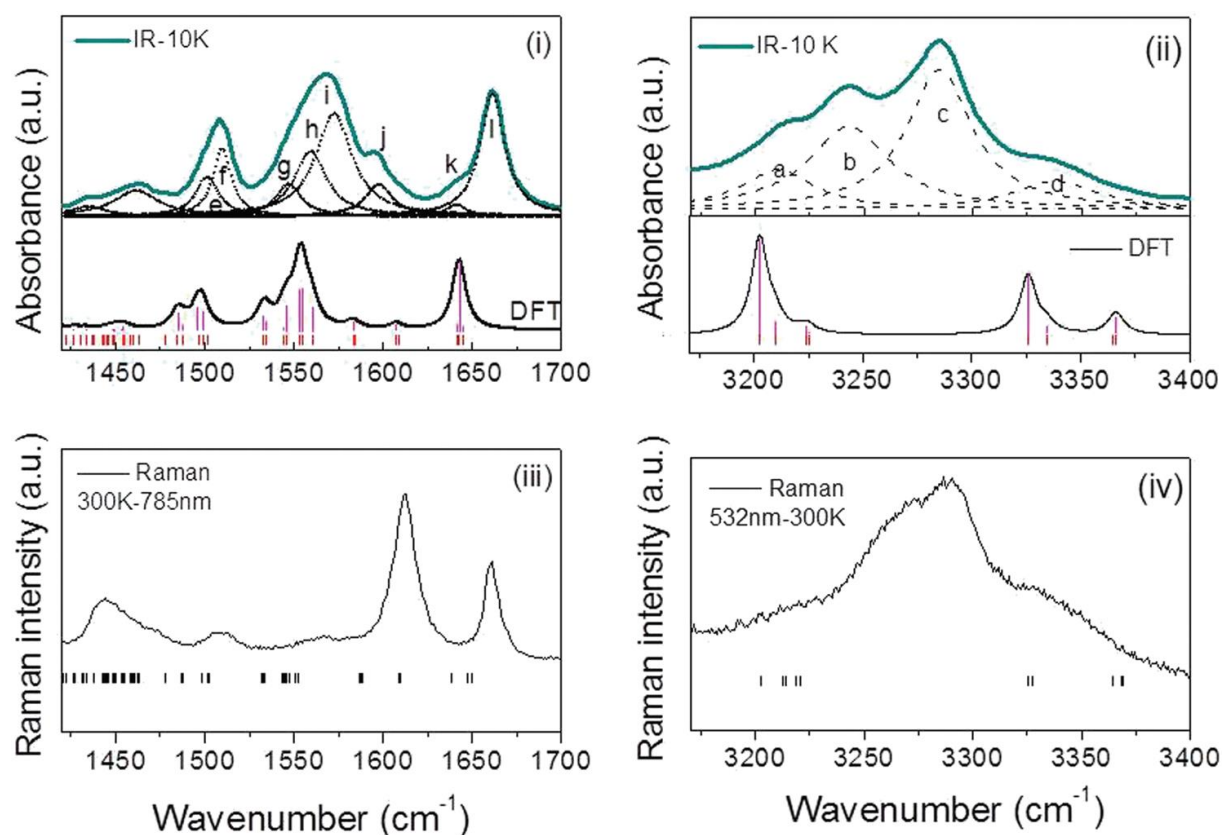
Fig. 2 Measured (10 K) and calculated infrared spectra for MUT located in the region of amide I and amide II (i) and in the region of amide A (ii). The deconvolutions of the experimental spectra at 10 K are obtained using Lorentzian bands. Experimental Raman spectra located in the region of amides I and II (iii) and amide A (iv) with calculated wavenumbers of Raman modes shown by vertical lines.
