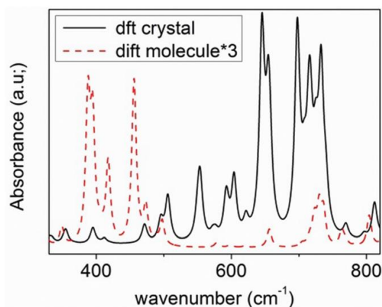
Fig. 5 Calculated spectra for the MUT crystal and isolated UT molecule, in the domains of amide V, thioamide V and thioamide I.
