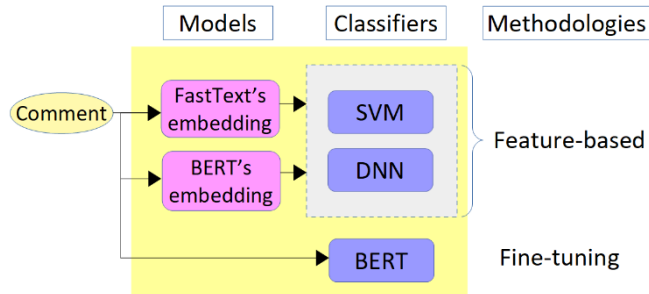
Fig. 1. Proposed methodologies
