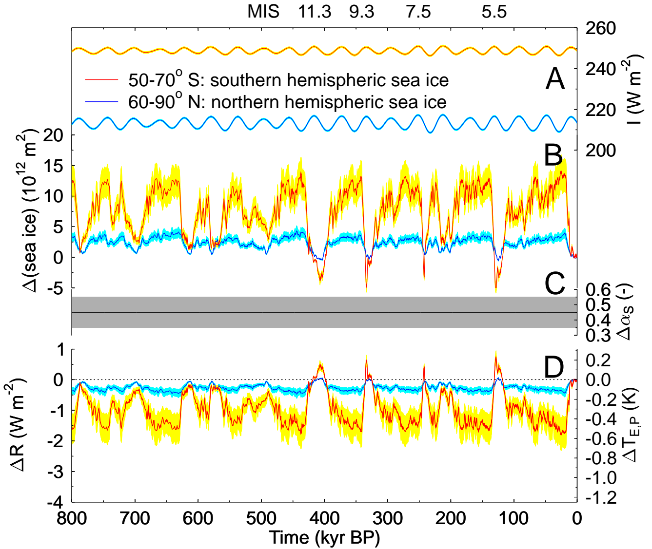
Figure 4: Sea ice-albedo feedback. (A) Annual mean local insolation at the top of the atmosphere I at 50-70^\circ \text{ S} and 60-90^\circ \text{ N} , the regions of SH and NH sea ice, respectively (Berger, 1978). (B) Area changes of sea ice. Estimates are based on (i) Antarctic temperature changes for the SH (Jouzel et al., 2007) and (ii) northern hemispheric temperature changes for the NH (Bintanja et al., 2005; Lisiecki and Raymo, 2005), linearly related to LGM to present sea ice area reconstructions. (C) Assumed changes in surface albedo \alpha_s from open ocean to sea ice. (D) Perturbation in the radiative budget caused by the sea ice-albedo feedback. The right y-axis shows the temperature anomalies \Delta T_{E,P} of the Planck feedback. The legend is valid for sub-figures A, B, and D.
