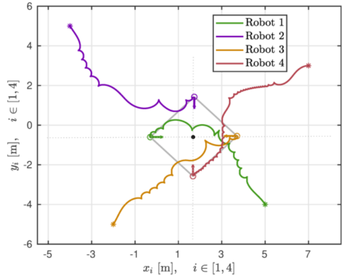
Fig. 3. Trajectories and formation of the network of mobile robots.
