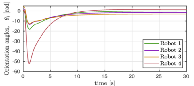
Fig. 4. Orientation of each mobile robot in the network.
