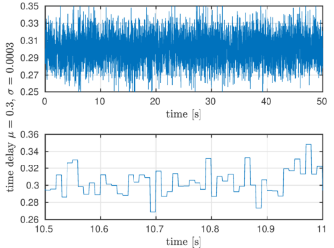
Fig. 2. Time delay in the network interconnection.
