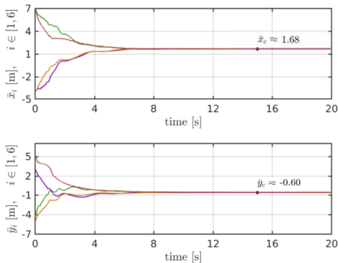
Fig. 5. Evolution of the relative positions z_i .
