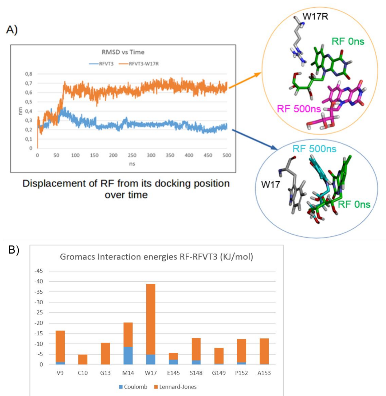
Figure 10. Molecular dynamics simulations on the complexes RFVT3-RF and RFVT3W17R-RF. A) Study of the displacement of RF. B) Average interaction energy between RF and the residues of the binding site. The contribution of the electrostatic (calculated by the Coulomb
