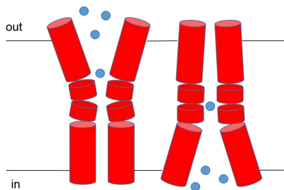
14 15 16 17 18 19 20 21 22 23 24 25 26 27 28 Figure 4. Schematic representation of the “rocker-switch” mechanism. 29 30
