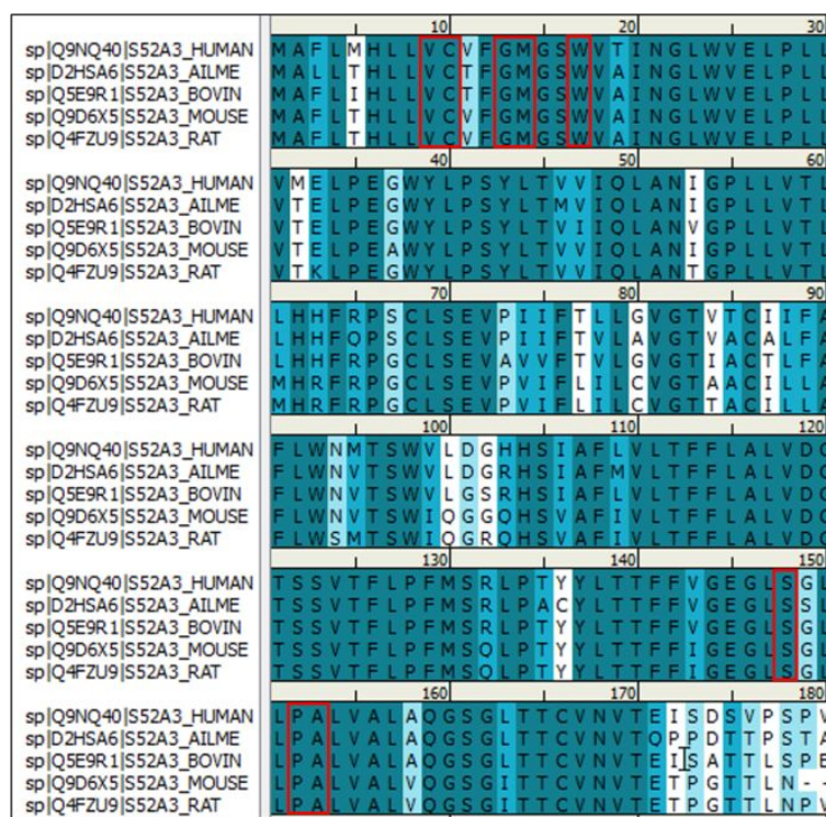
Figure 8. Alignment of RFVT3 sequences of different species. The residues of RF binding site are framed in red. The shades of blue indicate the similarity between compared residues (from
