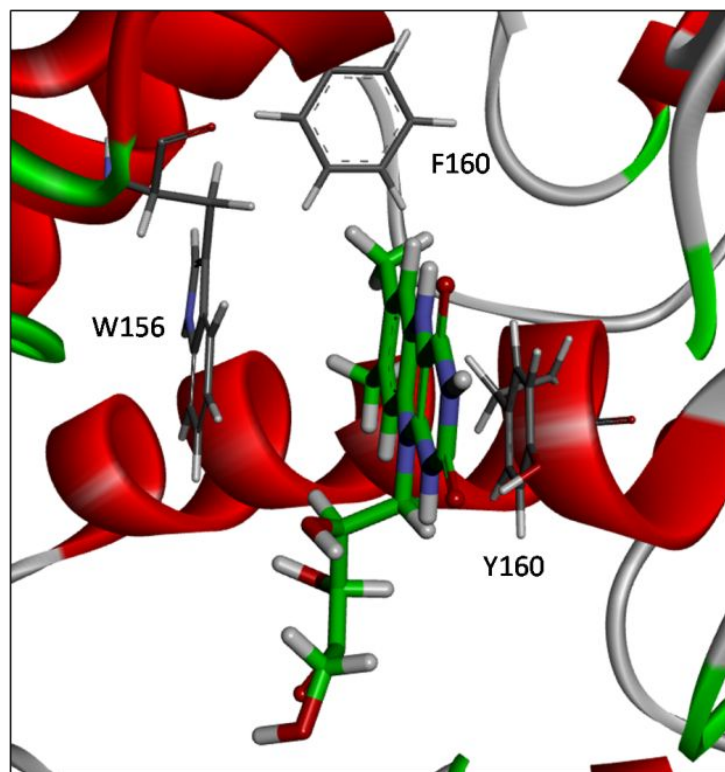
8 9 10 11 12 13 14 15 16 17 18 19 20 21 22 23 24 25 26 27 28 29 30 31 32 33 34 Figure 9. Binding mode of RF in the plasma carrier protein RCP (RX structure generously 35 provided by Pr. H.L. Monaco). 36 37
