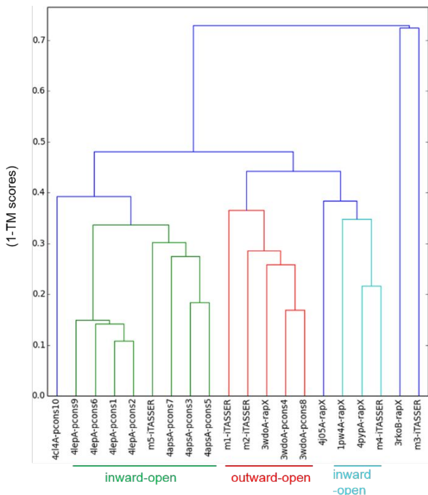
Figure 2. Dendrogram of the cluster analysis of RFVT3 models. For practical convenience, the y-axis indicates 1-TM scores. 3 groups (coloured green, red and cyan) and 4 outliers (blue) were revealed
