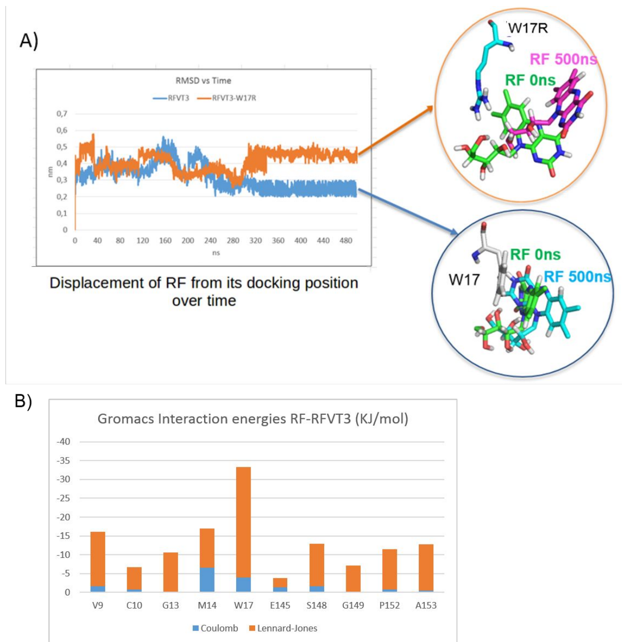
44 45 46 47 48 49 50 51 52 53 54 55 56 57 58 59 60 Figure 11. Replicate of Molecular dynamics simulations on the complexes RFVT3-RF and RFVT3W17R-RF. A) Study of the displacement of RF. B) Average interaction energy between RF and the residues of the binding site. The contribution of the electrostatic (calculated by the Coulomb potential) and Van der Waals (calculated by the Lennard-Jones Potential) are indicated by blue and orange bars, respectively.
