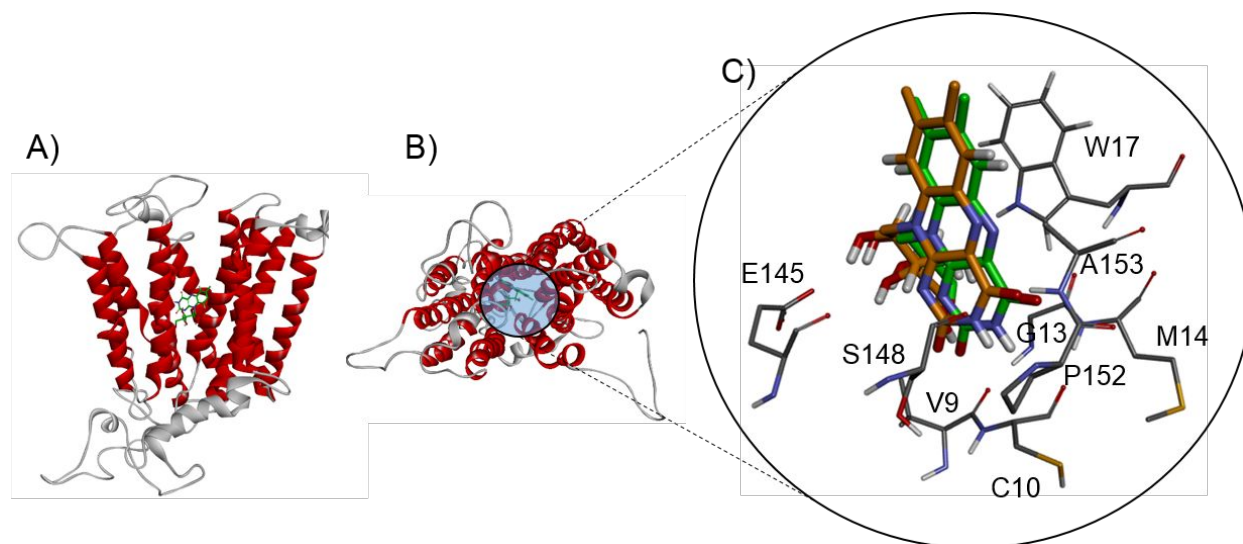
31 Figure 7. Docking of RF into RFVT3: A) Side view, B) Extracellular view and C) magnified 32 view of the potential RF binding mode detected by GOLD (RF is colored in green, red and blue) 33 and Autodock Vina (RF is colored in orange, red and blue) 34 35 36 37 38
