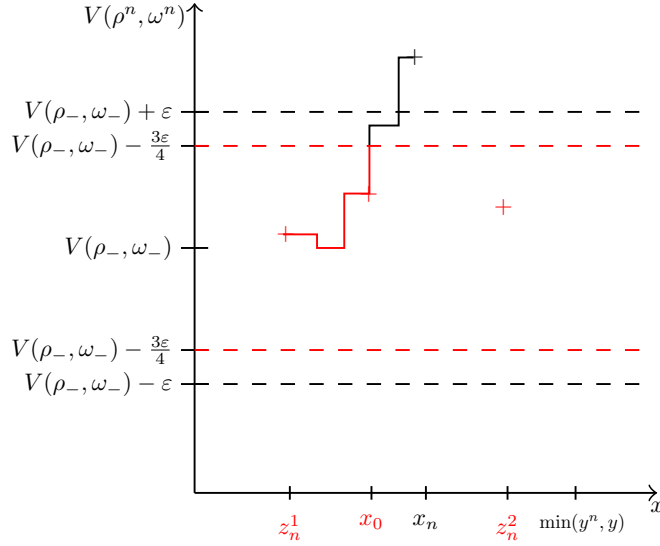
Figure 2: Illustration of V(\rho^n, w^n) if V(\rho_-, w_-) < V_b - \varepsilon and V(\rho^n(x_n), w^n(x_n)) > V(\rho_-, w_-) + \varepsilon with z_n^1 < x_0 < x_n < z_n^2 < \min(y^n, y) .
