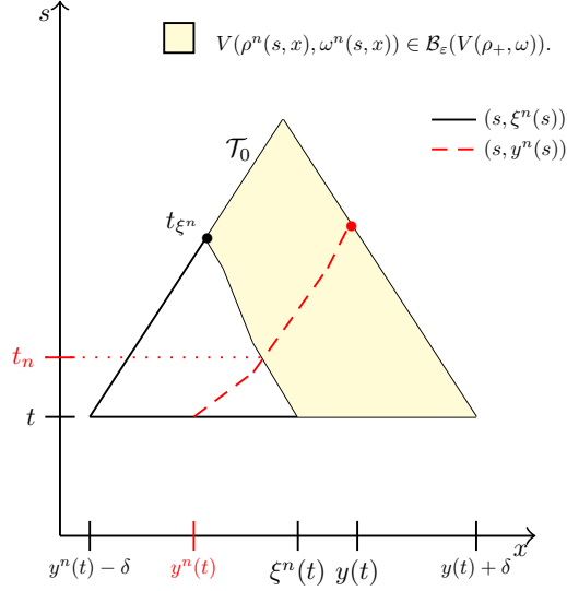
Figure 3: (\rho_-, \rho_+) \in (\rho^*(w), \rho_{\max}] with \rho_- \neq \rho_+ with y^n(t) < y(t) , n \geq n_1
