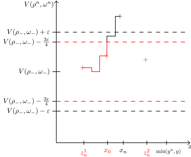
Figure 2: Illustration of V(\rho^n, w^n) if V(\rho_-, w_-) < V_b - \varepsilon and V(\rho^n(x_n), w^n(x_n)) > V(\rho_-, w_-) + \varepsilon with z_n^1 < x_0 < x_n < z_n^2 < \min(y^n, y) illustrationproof
