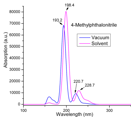
Fig. 10. As in Fig. 7, but for 4-methylphthalonitrile.
