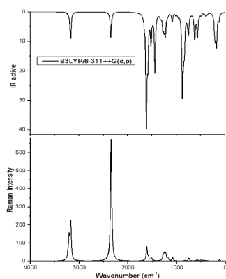
Fig. 3. The calculated IR activity and Raman activity vs. vibration frequency of 3,4-pyridinedicarbonitrile.
