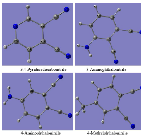
Fig. 1. Optimized geometrical structures of dyes 3,4-pyridinedicarbonitrile, 3-aminophthalonitrile, 4-aminophthalonitrile, and 4-methylphthalonitrile with atomic serial numbers.
