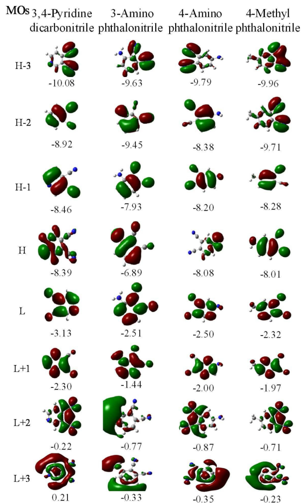
Fig. 11. Isodensity plots (isodensity contour = 0.02 a.u.) of the frontier orbitals of the dyes and corresponding orbital energies (in eV).
