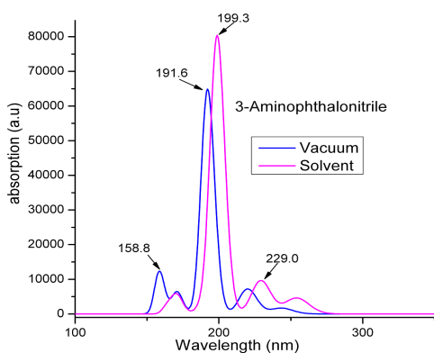
Fig. 8. As in Fig. 7, but for 3-aminophthalonitrile.
