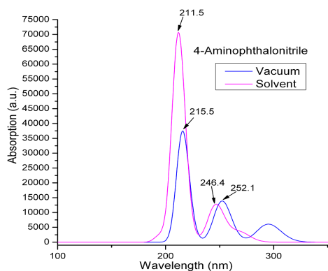
Fig. 9. As in Fig. 7, but for 4-aminophthalonitrile.
