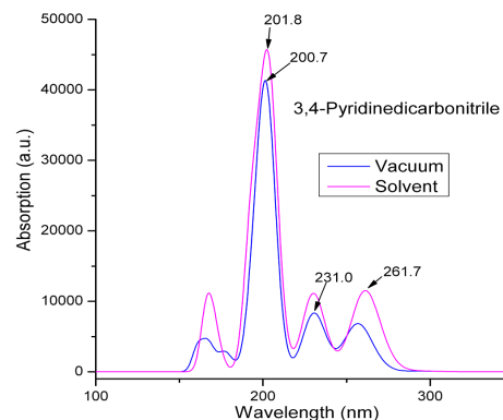
Fig. 7. Calculated electronic absorption spectra of 3,4-pyridinedicarbonitrile.
