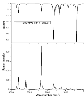
Fig. 5. As in Fig. 3, but for 4-aminophthalonitrile.
