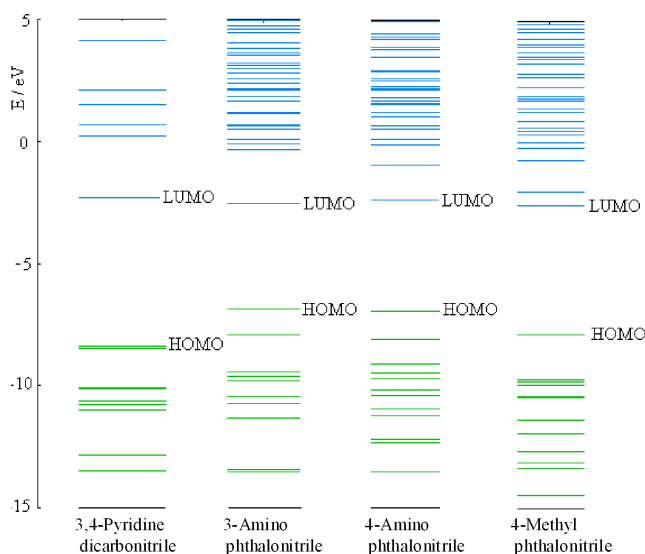
Fig. 2. The frontier molecular orbital energies of the dyes 3,4-pyridinedicarbonitrile, 3-aminophthalonitrile, 4-aminophthalonitrile, and 4-methylphthalonitrile.
