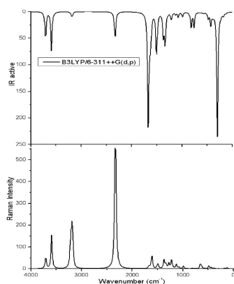
Fig. 4. As in Fig. 3, but for 3-aminophthalonitrile.
