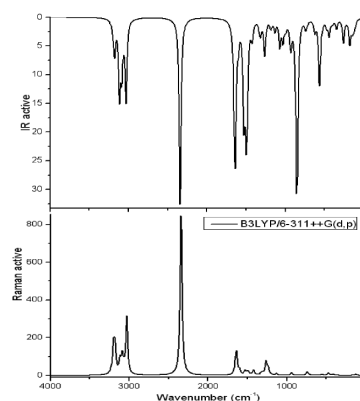
Fig. 6. As in Fig. 3, but for 4-methylphthalonitrile.
