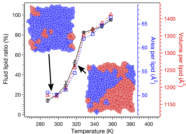
FIG. 3. Ratio of lipids in fluid state (black curve, vertical axis on the left), area per lipid (blue curve, vertical axis on the right) and volume per lipid (red curve, vertical axis on the right) as function of temperature. Two snapshots of the upper membrane leaflet, respectively taken at 288 and 318 K, are shown in the inset. The dark spots correspond to the 2d projection of the lipid center of masses. Boundaries between lipids result from the associated 2d Voronoi tessellation. Each cell color corresponds to the assignment of the ML, blue for the gel state and red for the fluid state.
