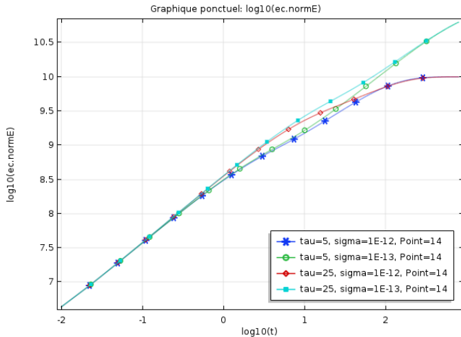
Figure 5 . Electric field (step reponse) vs time in front of the electrode with different time constant in Debye model and conductivity
