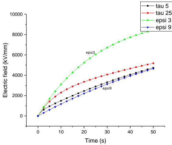
Figure 4 . Electric field (step reponse) vs time in front of the electrode. Blue/green: without Debye Model \epsilon_r = 9/3 . Black/red: with Debye Model \tau = 5/25(s)
