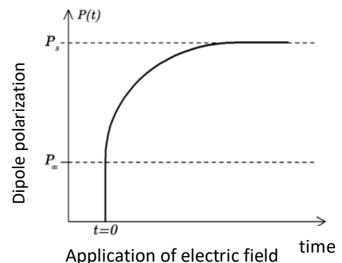
Figure 1 . Dynamic polarization for a step of E
