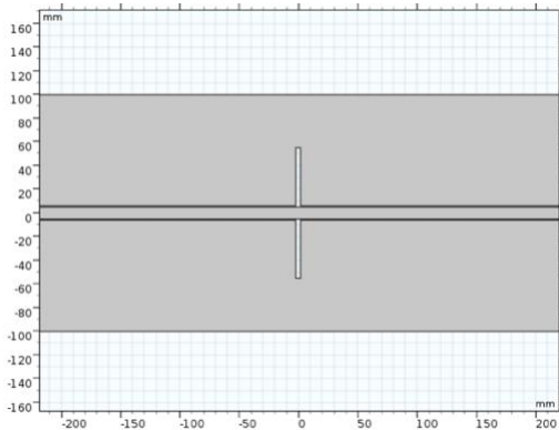
Figure 2 . The parallel-plane capacitor description in COMSOL
