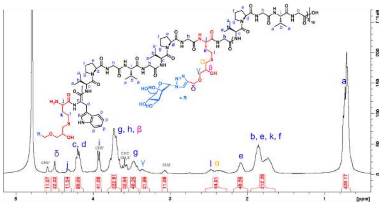
Figure S62. ^1\text{H} NMR spectrum of compound 4b (zoom) in \text{D}_2\text{O} .
