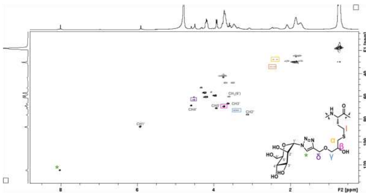
Figure S63. 2D NMR spectrum of compound 4b in \text{D}_2\text{O} , HSQC.
