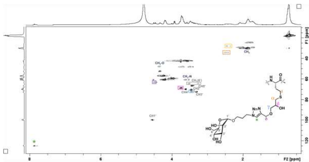
Figure S41. 2D NMR spectrum of compound 3d in \text{D}_2\text{O} , HSQC.
