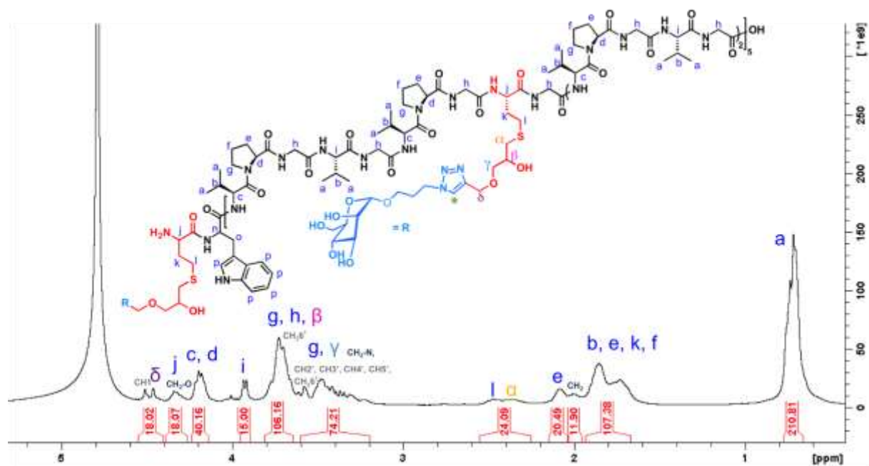
Figure S40. ^1\text{H} NMR spectrum of compound 3d (zoom) in \text{D}_2\text{O} .
