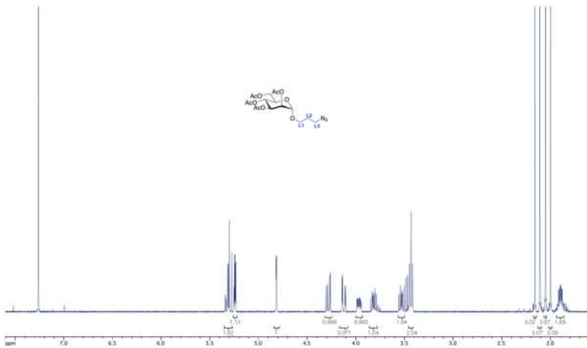
Figure S4. 1 H NMR spectrum of 3-azidopropyl (2,3,4,6-tetra- O -acetyl- \alpha -D-mannopyranoside) in CDCl 3 .
