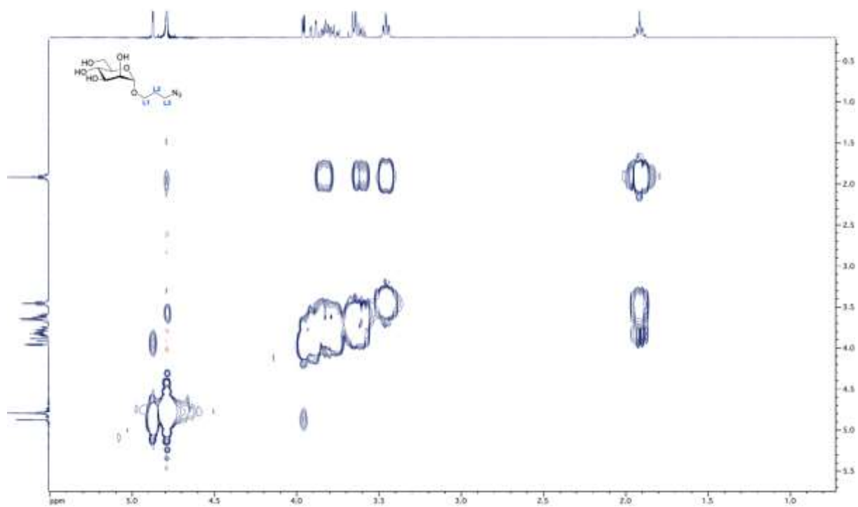
Figure S8. COSY NMR spectrum of 3-azidopropyl- \alpha -D-mannopyranoside in \text{D}_2\text{O} .
