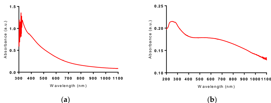
Figure 8. VIS-NIR absorbance spectrum of (a) Bi NPs produced from fs LAA and UV-VIS-NIR absorbance spectrum of (b) Bi nanosheets after fs LAW.
