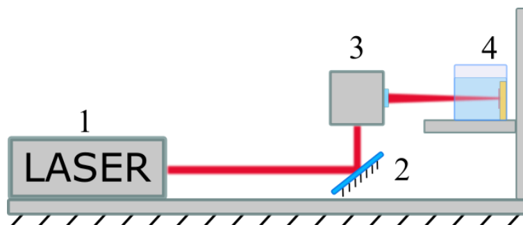
Figure 1. Schematic representation of the experimental setup for laser ablation. 1. a laser unit; 2. a mirror; 3. a galvanometric scanner and a focusing F-theta lens; 4. The ablation chamber with the Bi target submerged in liquid.
