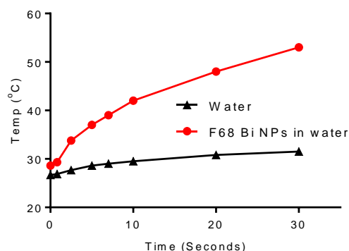
Figure 12. Photothermal heating of Pluronic® F68 coated Bi NPs, 10 days after transfer to water, using an 800-nm excitation source at 1-watt power.
