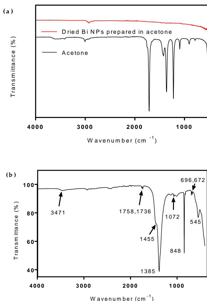
Figure 6. Fourier-transform infrared (FTIR) spectra of (a) Bi NPs produced from fs LAA and (b) Bi nanosheets after fs LAW.
