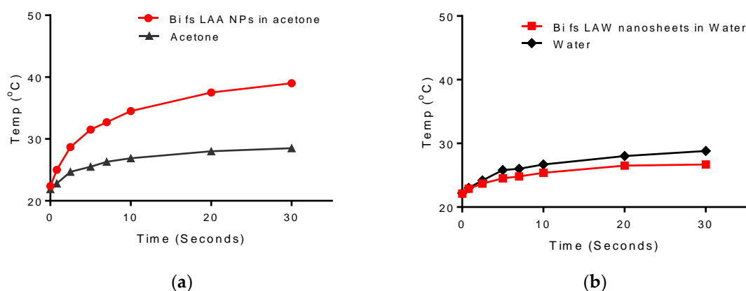
Figure 9. Photothermal heating of (a) Bi NPs produced from fs LAA and (b) Bi nanosheets after fs LAW, using an 800-nm excitation source at 1-watt power.
