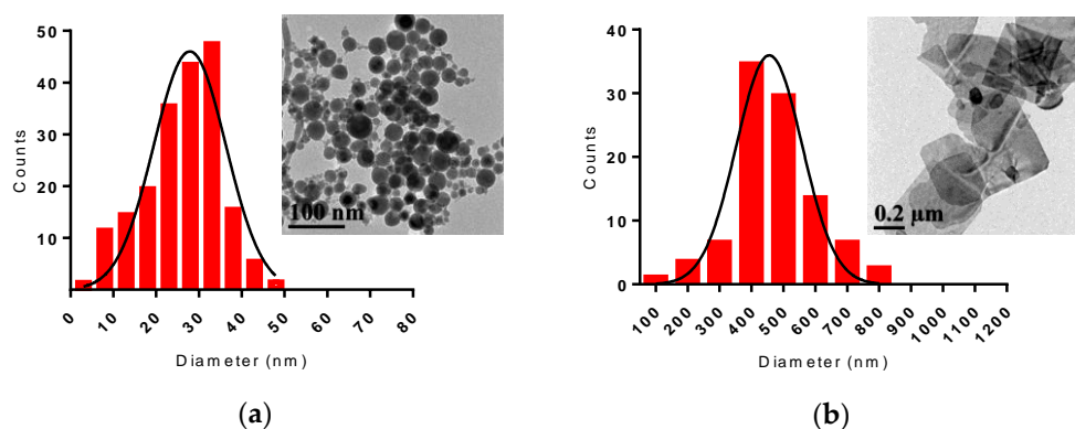
Figure 3. Size distributions and transmission electron microscopy (TEM) images of (a) Bi NPs produced from fs LAA and (b) Bi nanosheets after fs LAW.
