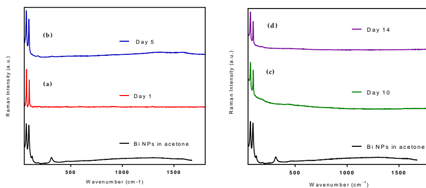
Figure 11. Raman spectra of Pluronic ® F68 coated Bi NPs (a) immediately after, (b) 5 days after, (c) 10 days after, and (d) 14 days after transfer to water, compared with as-synthesized Bi NPs in acetone.
