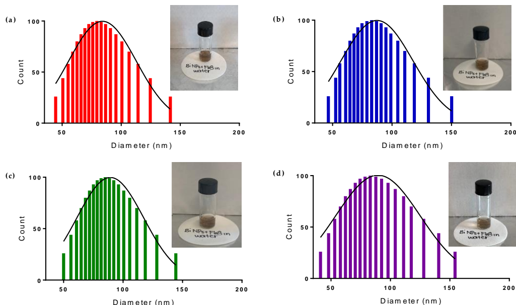
Figure 10. Colloidal solutions and size distributions, determined by Dynamic Light Scattering (DLS), of pluronic ® F68 coated Bi NPs (a) immediately after, (b) 5 days after, (c) 10 days after, and (d) 14 days after transfer to water.
