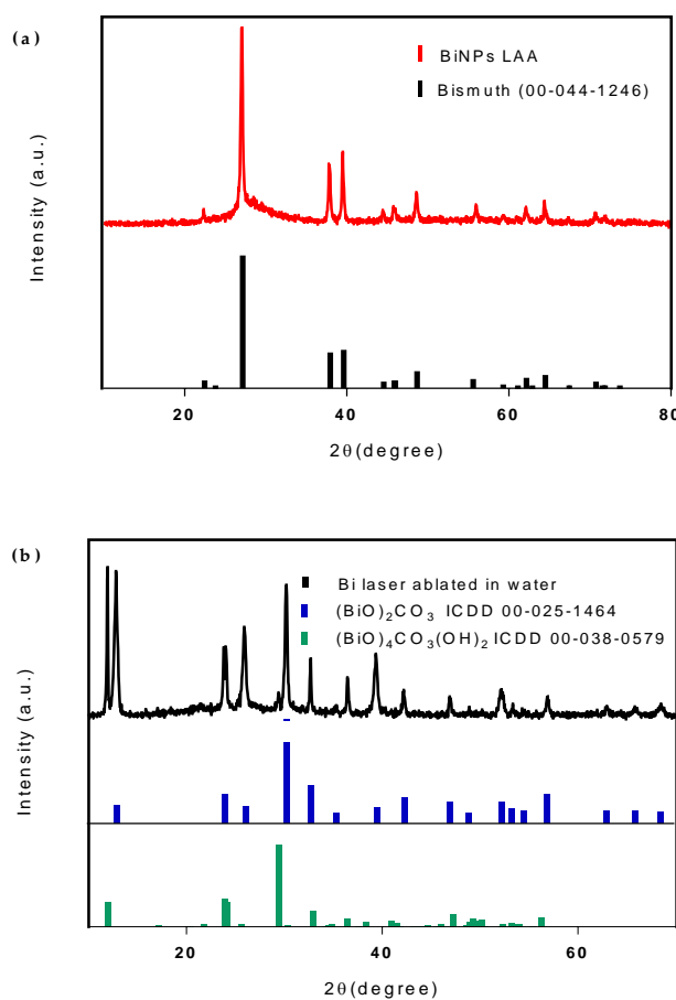
Figure 5. X-ray diffraction (XRD) patterns of (a) Bi NPs produced from fs LAA and (b) Bi nanosheets after fs LAW.
