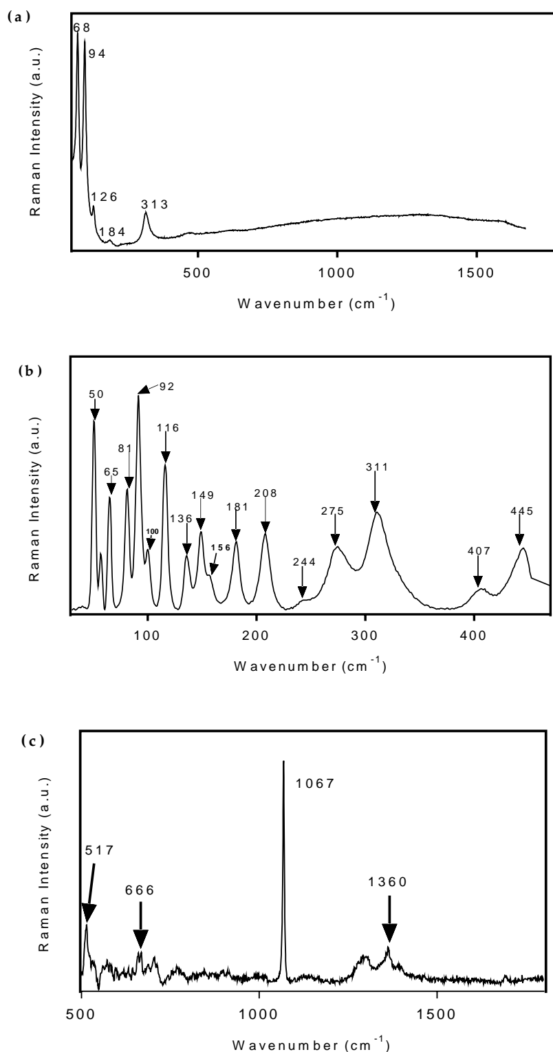
Figure 7. Raman spectra of (a) Bi NPs produced from fs LAA and (b,c) Bi nanosheets after fs LAW.
