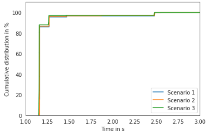
Figure 6: Cumulative distribution of the first uplink delay measured on the ED in s
