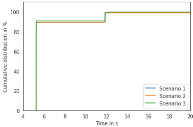
Figure 5: Cumulative distribution of the ED onboarding delay measured on the ED in s
