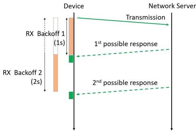
(a) Uplink/Downlink reception window in LoRaWAN
