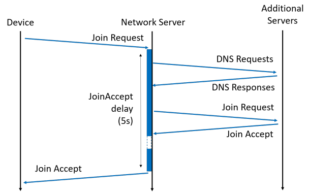
(b) OTAA Reception window in LoRaWAN
