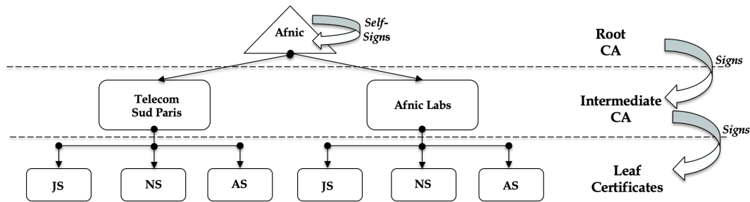
Figure 2: IoTRoam Certificate provisioning infrastructure
