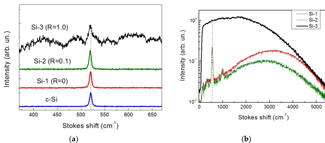
Figure 3. (a) Raman spectra of nc-Si sample obtained at different ratio of helium to nitrogen pressures, as well as one for c-Si substrate; (b) Raman and PL spectra measured in a wide range. Vertical dashed lines indicate the Raman line position (520.5 \text{cm}^{-1} ) for c-Si.
