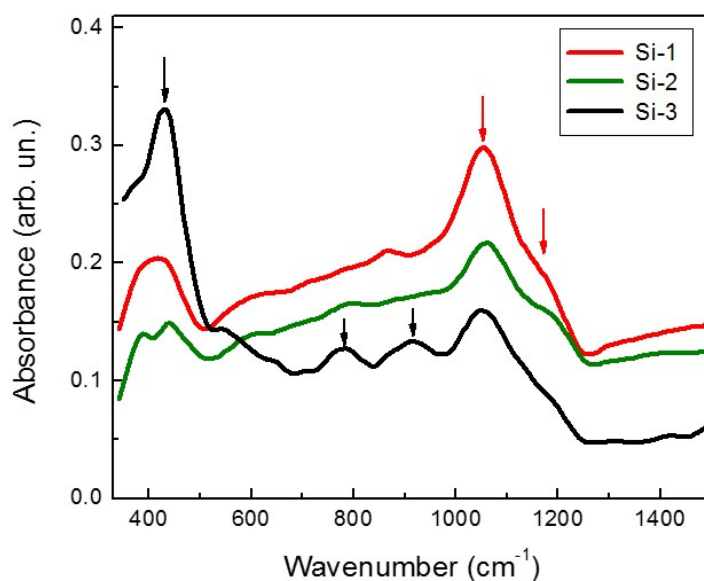
Figure 4. Fourier transform infrared (FTIR) absorption spectra of laser-ablated samples obtained at different ratio of helium to nitrogen pressures. Vertical red and black arrows indicate the spectral position of the Si-O and Si-N bonds, respectively.
