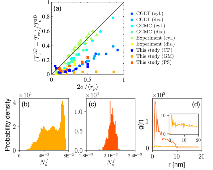
FIG. 1. The degree of confinement represented by (a) shift in capillary critical temperature T_{cc} as a function of the ratio 2\sigma/\langle r_p \rangle . Previous simulations (circle) and experimental (triangle) data from the literature [58] along with our results (square) for all the considered cylindrical pores (CP), porous solids (PS), and granular media (GM) and for various space discretizations a_0 , where a_0 \sim \sigma . (b), (c) N_s^f(r = 20 nm) of GM and PS, respectively, for structure C . (d) Partial radial distribution function for a fluid site at the pore-solid interface with a connected path to a solid site at the pore-solid interface.
