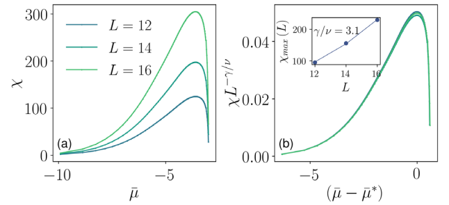
FIG. 4. (a) Susceptibility for structure C and \bar{T} = 1.5 for volumes of length L = 12 ( N = 217 ), L = 14 ( N = 126 ), and L = 16 ( N = 125 ). (b) Collapse of the susceptibility curves (inset: a power law fit to estimate \gamma ).
