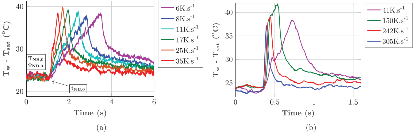
Fig. 16. a. Slow temperature ramps and b. Steep ramps as measured by the infrared camera for Re = 27\,000 and, \Delta T_{sub}=14\text{ °C} , Ja_{sub}=22 . (For interpretation of the references to colour in this figure legend, the reader is referred to the web version of this article.)
