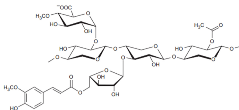
Figure 11. Structure of hemicellulose [156] (Reprinted from Water Extraction of Bioactive Compounds, From Plants to Drug Development , Siti Machmudah, Wahyudiono, Hideki Kanda, Motonobu Goto, Chapter 3—Hydrolysis of Biopolymers in Near-Critical and Subcritical Water, 69–107, Copyright 2017, with permission from Elsevier).
