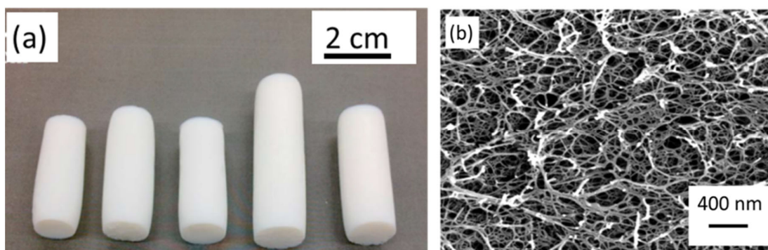
Figure 18. \kappa -carrageenan aerogels prepared via gelation with KSCN: a) monoliths made from solutions of polymer concentration (from left to right) 1; 1.5; 2; 2.5 and 3 wt%, b) scanning electron microscopy image of the fractured surface of aerogel made from 1 wt% solution (adapted from [257]).
