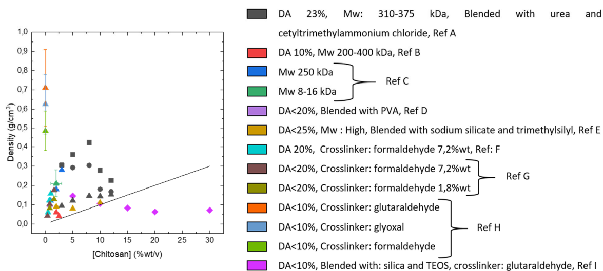
Figure 20. Variation of the density as a function of the chitosan concentration. Methods of drying are represented by squares for ambient drying, circles for drying at 65^\circ\text{C} , diamonds for freeze drying and triangles for supercritical drying. The solid line represents the density for pure chitosan materials without shrinkage and without mass loss. Ref A: [273], Ref B: [274,275], Ref C: [276], Ref D: [277], Ref E: [278], Ref F: [279], Ref G: [280], Ref H: [281], Ref I: [282].
