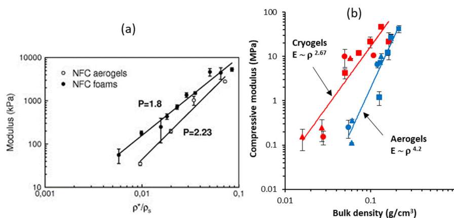
Figure 6. Compressive modulus as a function of (a) relative density for aerogels and foams based on CNF [85] (Reprinted from Composites Science and Technology , 71, Sehaqui, H.; Zhou, Q.; Berglund, L.A. High-porosity aerogels of high specific surface area prepared from nanofibrillated cellulose (NFC), 1593–1599, Copyright 2011, with permission from Elsevier) and (b) as a function of bulk density for aerogels and cryogels (or foams) based on cellulose II [89].
