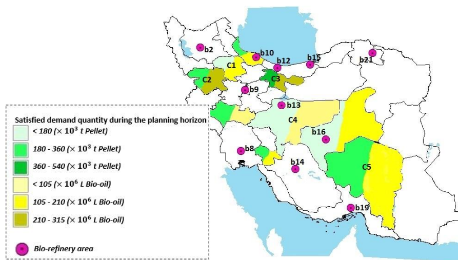
Figure 9: Deterministic model
