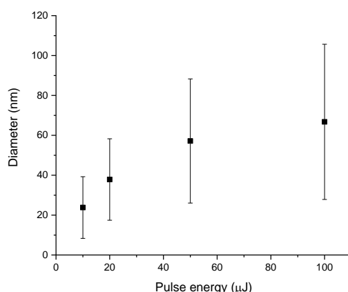
Figure 4. Diameter of spherical Sm oxide NPs obtained by laser ablation at different pulse energies. Data points and scale bars represent mean size and standard deviations from lognormal fit of number-weighted size histograms.
