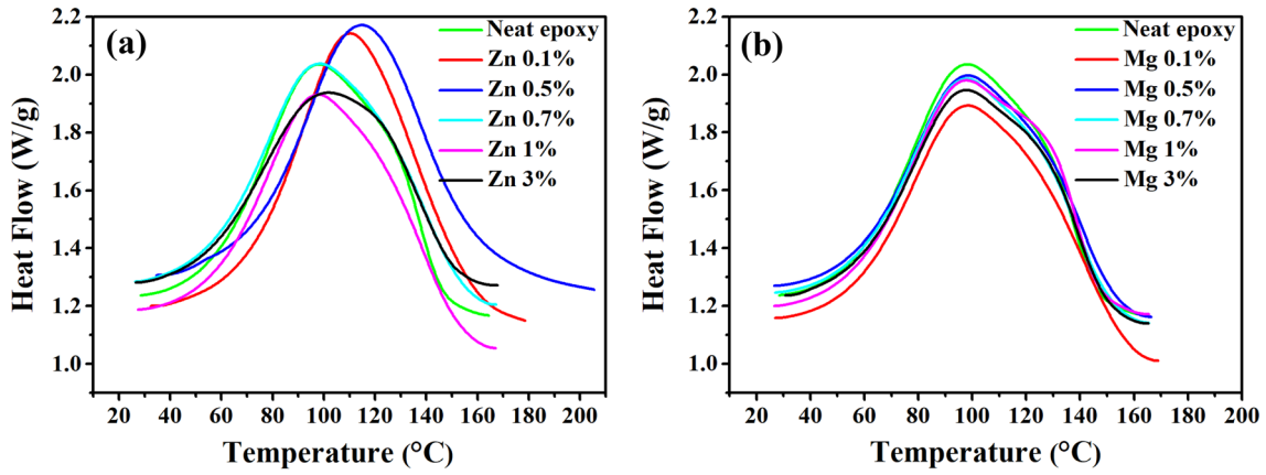
Fig. 5 Non-isothermal DSC thermograms of epoxy nanocomposites containing various contents of a Zn–Al–LDH and b Mg–Al–LDH at heating rate of 10 °C/min
