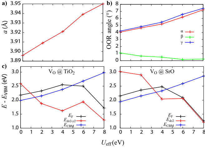
FIG. 7. Calculated SrTiO 3 atomic structure parameters and electronic band levels as a function of the U_{\text{eff}} parameter: a) Lattice parameter a calculated for the cubic bulk STO and used as the in-plane lattice parameter for the strained 2 \times 2 \times 5 bulk supercells and for the interface studies. b) OOR angles calculated when the V_{\text{O}} is located in a TiO 2 atomic layer in the 2 \times 2 \times 5 supercell. The angles \alpha , \beta and \gamma are given respectively according to the 3 crystallographic axes a[100] , b[010] and c[001] , which are parallel to the Ti-O chemical bounds. The values are averaged on every oxygen octahedra not included in the TiO 2 layer containing the V_{\text{O}} . c) Energy band levels at the \Gamma high-symmetry point. We define as E_{\text{VBM}} and E_{\text{CBM}} the energies of the states delimiting the band gap for the non-defective SrTiO 3 bulk compound, i.e. respectively the highest occupied O-p band and the lowest unoccupied Ti- d_{xy} band. The given values are calculated when the V_{\text{O}} is located in a TiO 2 (left) or SrO (right) (001) atomic layer and the red curve corresponds to the energy of the d_{x^2-y^2} or d_{z^2} gap state.
