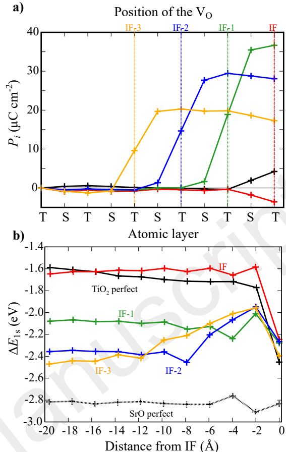
FIG. 4. a) Local electric polarization P_i as a function of the position of the V_O and of the atomic layer i (T is for \text{TiO}_2 and S for SrO) and b) variation of the O-1s energy level as a function of the distance to the interface. The value \Delta E_{1s} is given according to the energy level calculated for the bulk STO.
