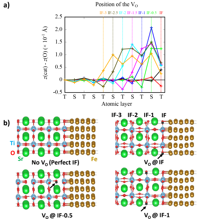
FIG. 3. a) Cation-oxygen buckling; the black curve corresponds to the reference structure without V_O . The letters "T" and "S" represent respectively the TiO_2 and SrO atomic layers. b) Atomic structure of the Fe/SrTiO 3 without any oxygen vacancy V_O and with one oxygen vacancy in three different positions.
