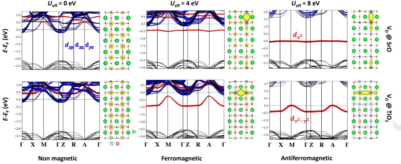
FIG. 8. Band structures and charge densities associated to the electronic states in the energy range between E_F - 1.5 eV and E_F , calculated for different values of U_{\text{eff}} and the oxygen vacancy located in a \text{TiO}_2 or \text{SrO} (001) atomic layer.
