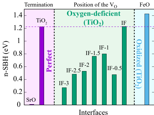
FIG. 6. Summary of the different n-type Schottky barrier heights (SBH) calculated for the perfect SrO- and TiO 2 -terminated interfaces (left) and for the TiO 2 -terminated interface with an oxygen vacancy (center) or an oxidized FeO layer (right).
