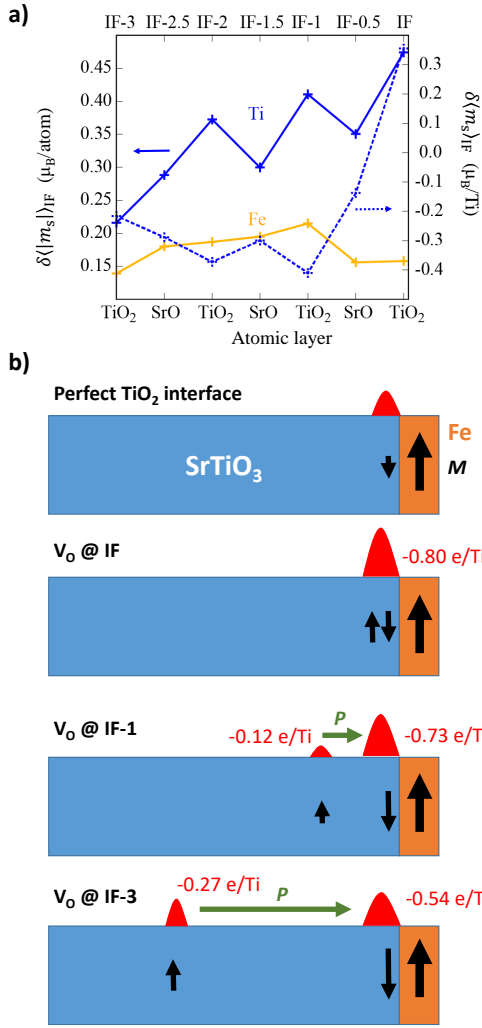
FIG. 10. a) Variation of the averaged spin magnetic moment \langle m_s \rangle (dotted line, right) and its absolute value (solid line, left) |m_s| of the interfacial Ti and Fe atoms as a function of the position of the oxygen vacancy near the TiO 2 -terminated interface. The values are given relatively to the moment of the same atoms at the perfect interface. b) Schematic representation of the charge localization (in red), leading to the emergence of an electric polarization P (green arrow) and of the magnetic ordering (black arrows) as a function of the V O position.
