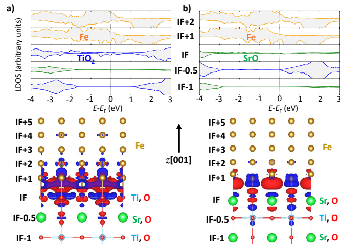
FIG. 1. (top) Layer-resolved densities of states (LDOS) of the (001) atomic planes and (bottom) charge density difference near the a) TiO 2 - and b) SrO-terminated interfaces (IF). The charge density difference is defined by the formula \Delta\rho = \rho_{\text{HS}} - (\rho_{\text{STO}} + \rho_{\text{Fe}}) , where \rho_{\text{HS}} , \rho_{\text{STO}} and \rho_{\text{Fe}} are respectively the charge densities for the heterostructure, the STO and the Fe layers. Red area corresponds to a positive \Delta\rho , while blue area is for negative values.
