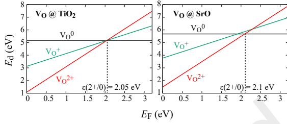
FIG. 9. Formation energies E_d(V_O^g) of an oxygen vacancy located either in a \text{TiO}_2 (left) or a \text{SrO} (right) atomic layer as a function of the position of the Fermi level E_F . The energies were calculated using the 2 \times 2 \times 5 bulk supercell.
