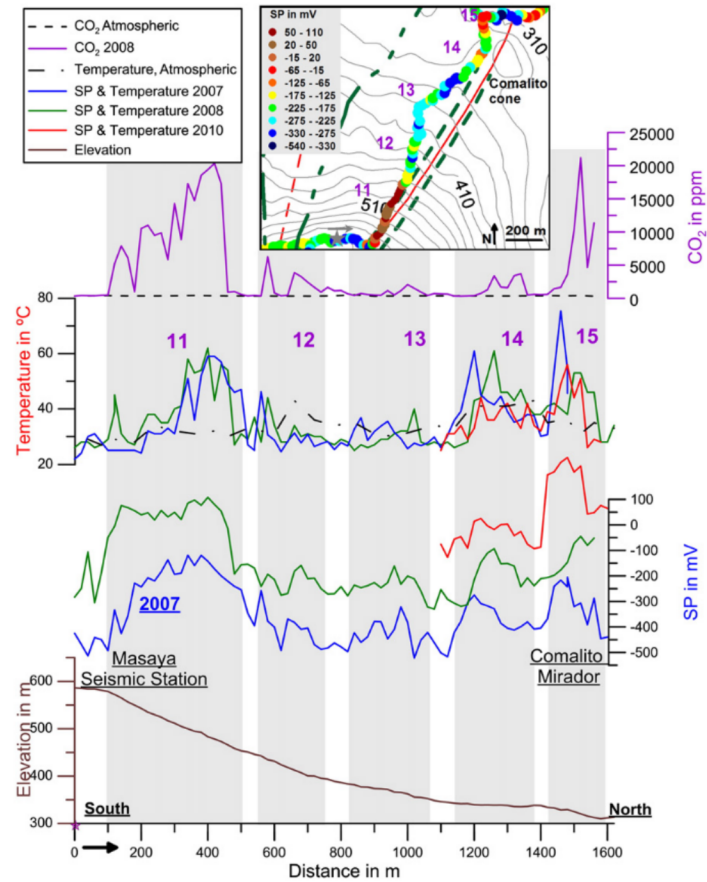
Fig. 6. Self-potential, CO 2 concentration, temperature and topography of the survey profile across the north flank of Masaya cone to the solfatare of Comalito measured in 2007 and 2008. All self-potential profiles are referenced to the same base station at the Laguna de Masaya, which is assumed to be stable over time and to which a 0 mV value has been attributed to facilitate comparison of the different surveys. The purple numbers (and shaded areas) represent the anomalies reported in Table 1. Sampling step is 20 m. The star indicates the beginning and end of the profile. (For interpretation of the references to color in this figure legend, the reader is referred to the web version of this article.)
