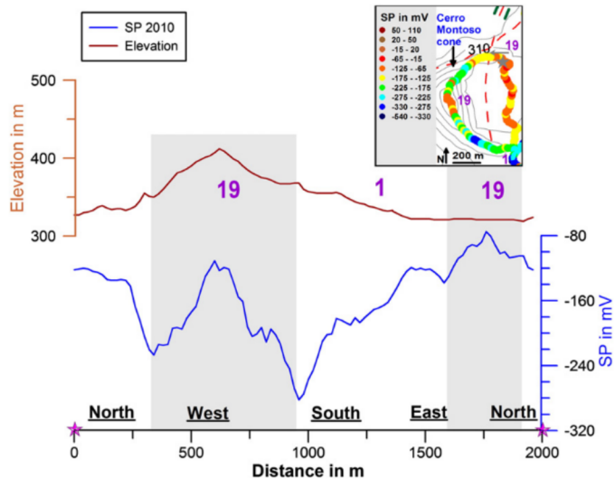
Fig. 8. Self-potential profile of the survey across Cerro Montoso cone measured in 2010. All the self-potential profiles have been corrected for drift and level has been shifted to
