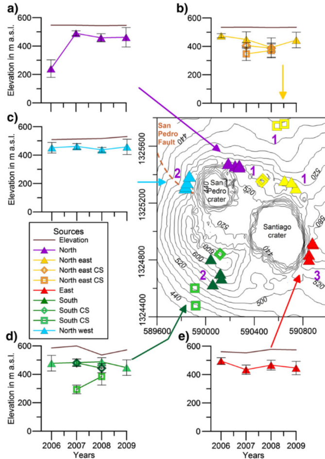
Fig. 9. Water depths between 2006 and 2009 on Nindiri cone. Horizontal GPS coordinates and depths of the water are obtained by multi-scale wavelet tomography applied on the self-potential survey loop. Triangles represent depths calculated from the MWT analysis of the Nindiri survey loop (Fig. 5). Squares and diamonds are calculated depths from the MWT analysis of a Nindiri cross-section SP profile (from Mauri et al., 2010). All depths are presented in Appendix 1. (For interpretation of the references to color in this figure legend, the reader is referred to the web version of this article.)
