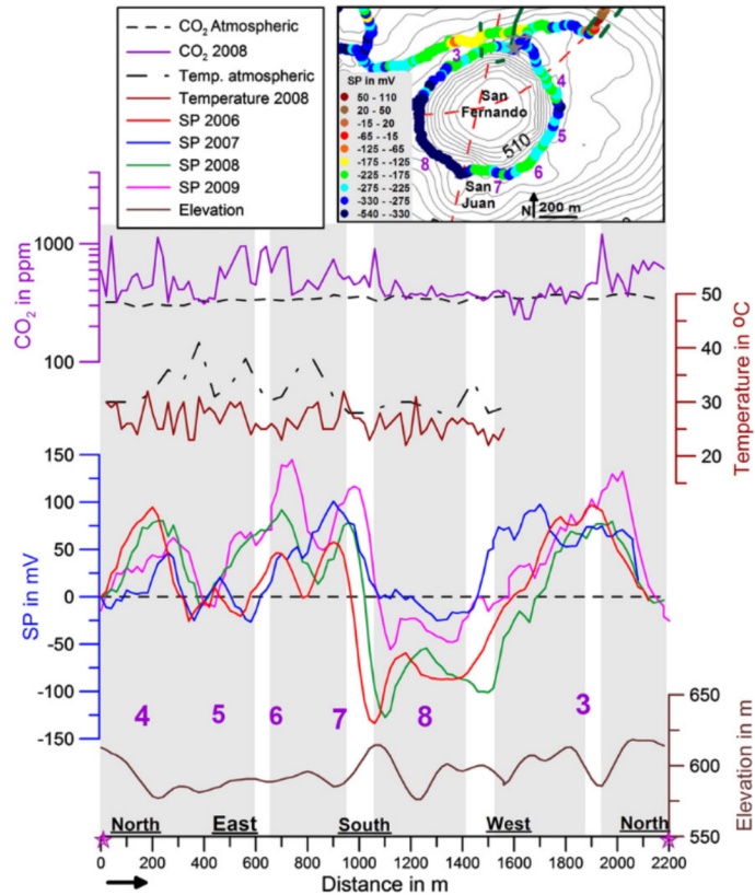
Fig. 5. Self-potential, CO 2 soil concentration, ground temperature and topography of the survey profile around Masaya crater measured between 2006 and 2009. All self-potential profiles are referenced to the same base station on the north rim of the crater of Masaya, which is assumed to be stable over time and to which a 0 mV value has been attributed to facilitate comparison between different surveys. The purple numbers (and shaded areas) represent the anomalies reported in Table 1. Sampling step is 20 m. The star indicates the beginning and end of the profile. (For interpretation of the references to color in this figure legend, the reader is referred to the web version of this article.)
