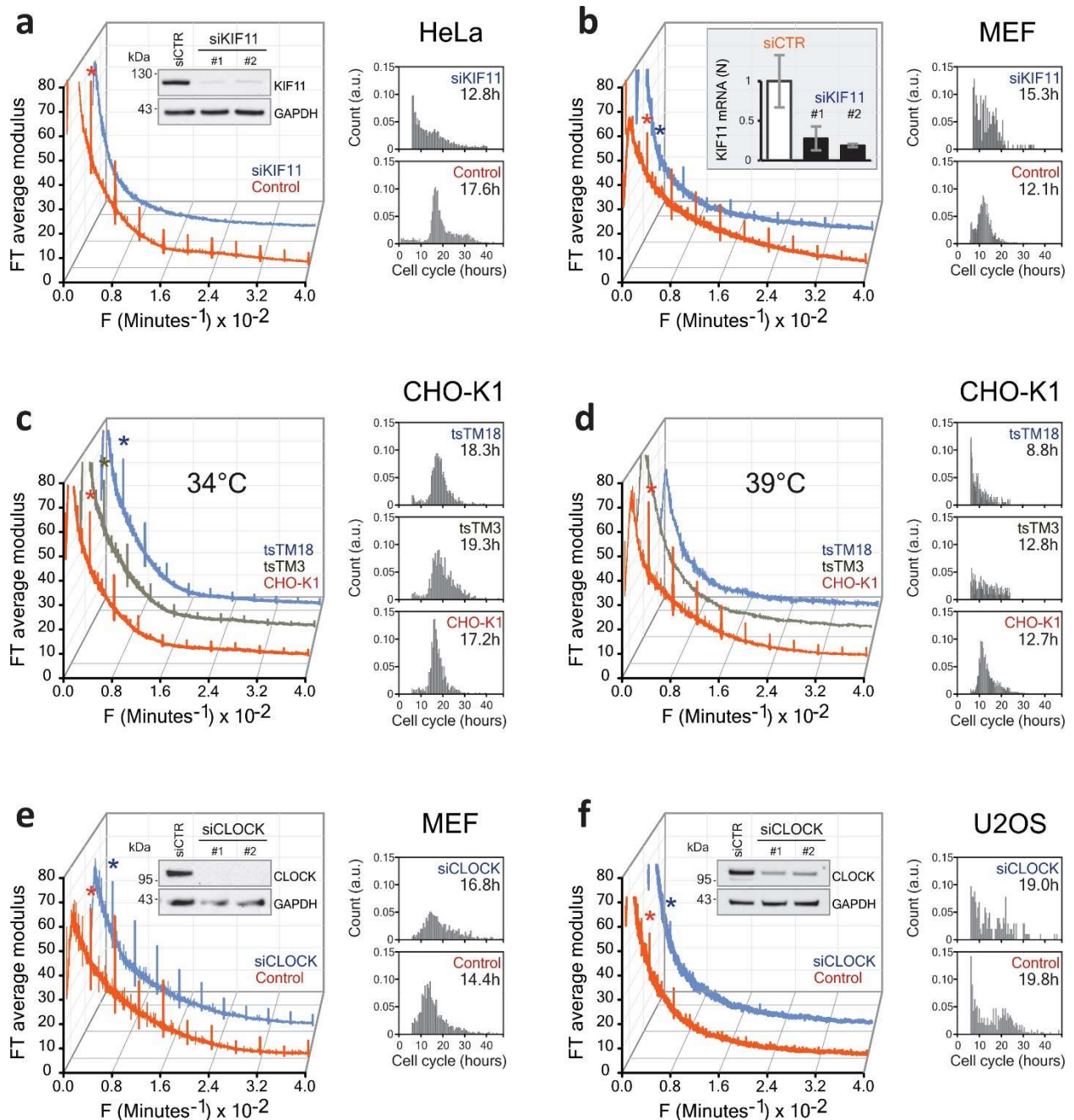
Figure 3. Relationship between the Rhythm, Cell cycle and Circadian Clock. (a) Cell cycle arrest by siKIF11 treatment in HeLa cells suppresses the 4 h rhythm. Western blots (in insert ) confirm the inhibition of KIF11 expression (the effect of two specific siRNAs is compared to non-specific siCTR). (b) Effects of the cell cycle inhibition on the 4 h rhythm via siKIF11 treatment in MEF : The rhythm is not suppressed . Quantitative PCR analysis (in insert) shows the inhibition of KIF11 expression by two specific siRNAs in MEF. To the right of (a) and (b) we show the distributions of the cell cycle lengths corresponding to the two data sets. (d) Effects of cell cycle inhibition in temperature-sensitive CHO-K1 mutants at 39°C , compared to the permissive 34°C temperature
