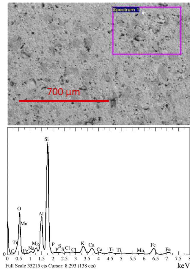
FIG. 1. SEM-EDS analysis of the surface ceramic. Top: SEM image perpendicular to the sample surface, pores correspond to black spots in the image; bottom: EDS spectrum of the ceramic.
