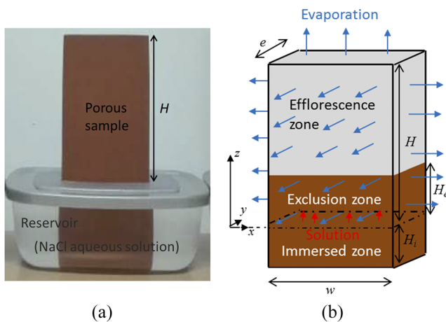
FIG. 2. (a) Porous sample partially immersed in the bottom reservoir at the beginning of the experiment and (b) sketch of the studied system with the main notations.
