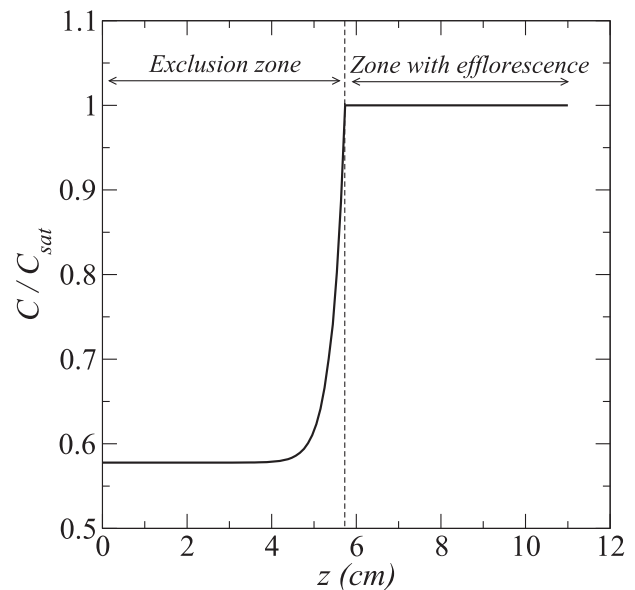
FIG. 8. Typical average ion mass fraction profile along the sample height computed from Eq. (A11) in the Appendix for C_0 = 0.15 .
