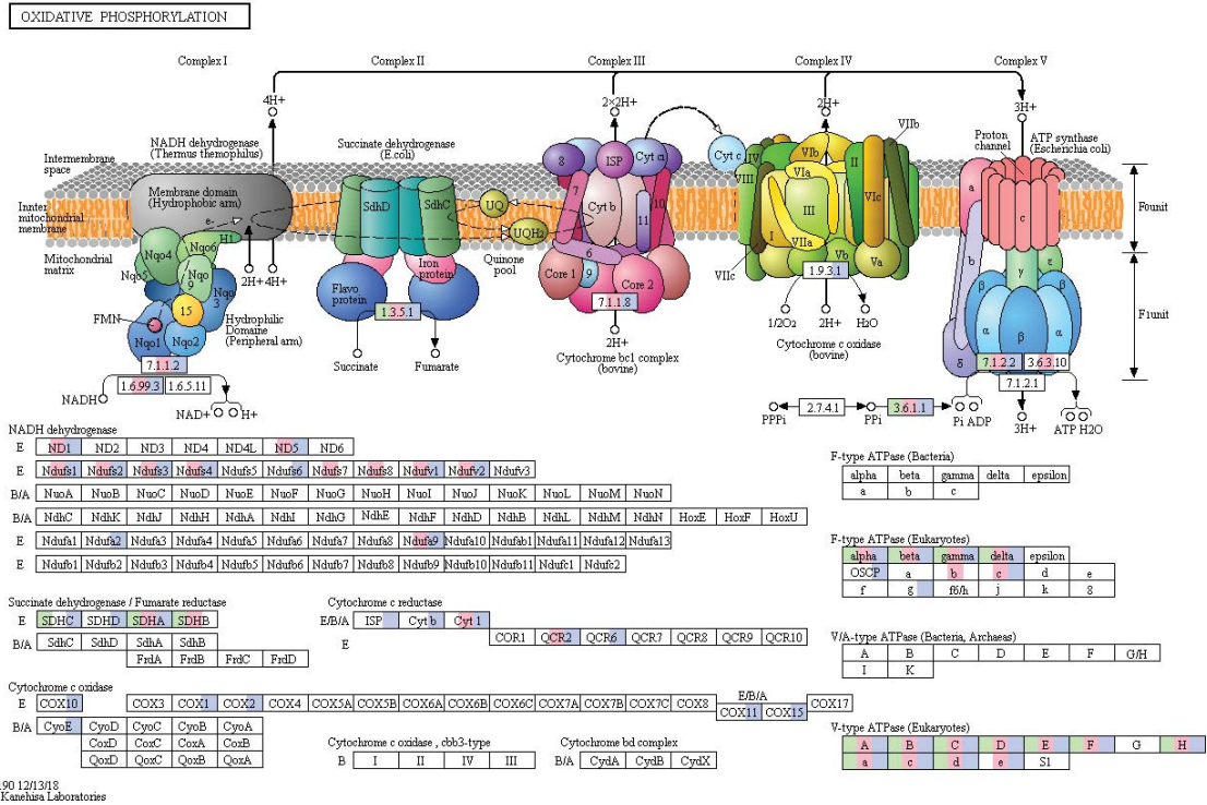
Fig. S8. Oxidative phosphorylation pathways of H. salmonicola , M. squamalis and K. iwatai . The proteins identified in the mitochondrial genome and the transcriptome of H. salmonicola , M. squamalis and K. iwatai are indicated in green, red and blue, respectively. The absence of a protein is indicated in white. Results corresponding to pseudogenes in H. salmonicola (i.e., NuoI/comp_48827 and NduF1/comp_72978) were removed and therefore appear white in this figure.
