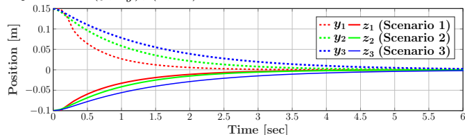
Fig. 4: Convergences of x, y, z under different scenarios.
