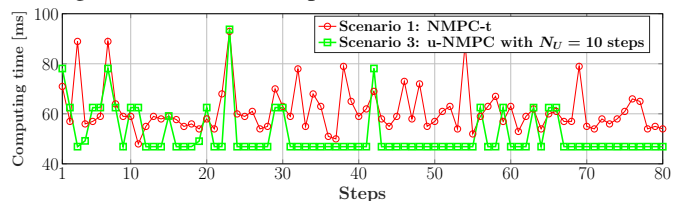
Fig. 9: Computation time under experiments using Pyomo in Python 3.0.
