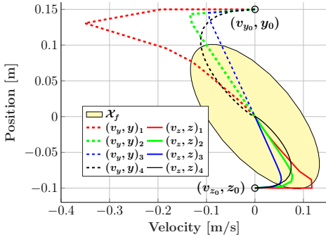
Fig. 3: Terminal region \mathcal{X}_f (approximated illustration) and the trajectories (y, v_y), (z, v_z) under different scenarios.
