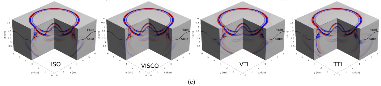
Figure 4: Modeling results of 3D bilayered models. (a) Seismogram comparison with results of SPECIFEM3D (Peter et al., 2011) in the isotropic case, where the receiver is located on the seabed with the x - and y - offset of 2.8 km and 0.1 km. Panels (b) and (c) are comparisons of pressure records and vertical displacement snapshots in the isotropic, viscous-isotropic, VTI and TTI cases, respectively.
