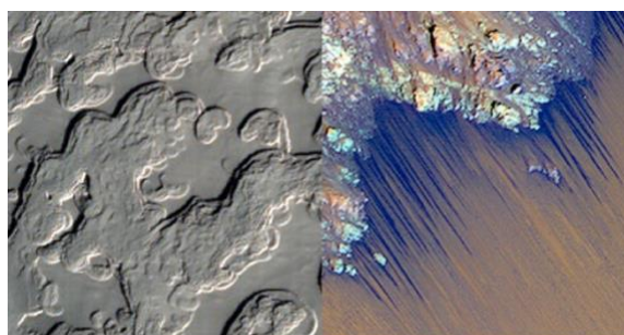
Figure 1: SPRC CO 2 ice features, ESP_012784_0935 (left) and RSL surface features, ESP_034830_1670 (right). Both from HiRISE, NASA/JPL/UoA
