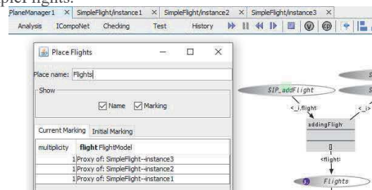
Fig. 2. Marking of the place "Flights" of the model PlaneManager1.
