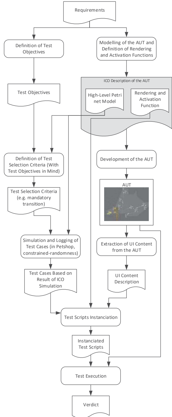
Fig. 6. The Process of Random-Model Based Testing of applications featuring dynamic instantiation of GUI widgets.
