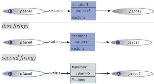
Fig. 3. Example of a transition with a pre-condition. Initially, place0 contains 9 tokens, 2 of which carrying a value of 5.
