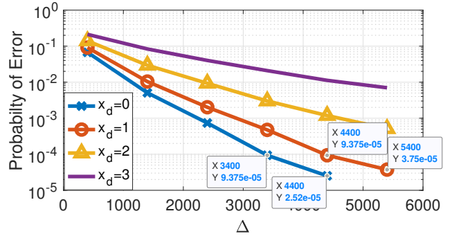
Fig. 2. Average probability of error with different initial position, x_d \mu m , of the receiver with a region [x_d \mu m, x_d + 1 \mu m] and varying quantity of molecules \Delta .
