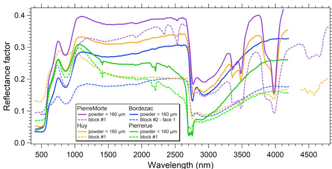
Figure 5: Vis-NIR reflectance spectra of the powder (grain size < 160 \mu\text{m} ) and a raw block for Pierremorte, Bordezac, Huy, and Pierrerue.
