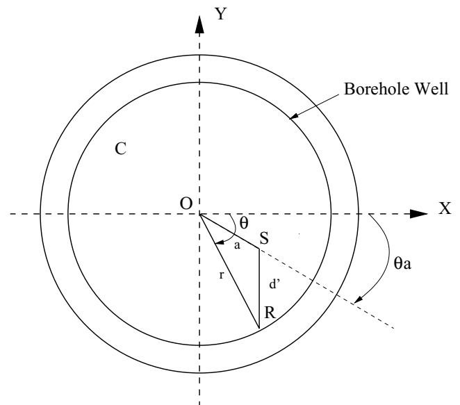
Figure 6. Principle of the demodulation (DEM) correction. When the tool is off-centred (S position) it induces a sinusoidal shape on the recorded data. The tool is located in O if it is well centred in the hole.
